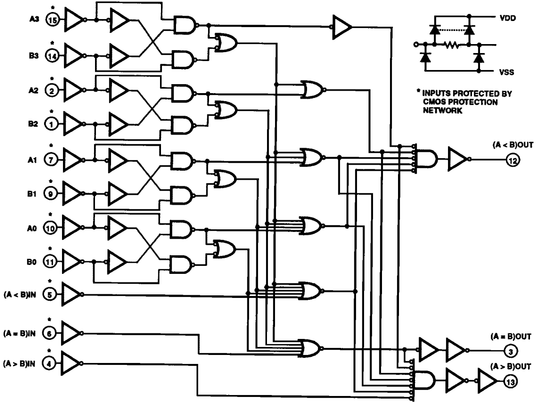
FIGURE 1. LOGIC DIAGRAM
