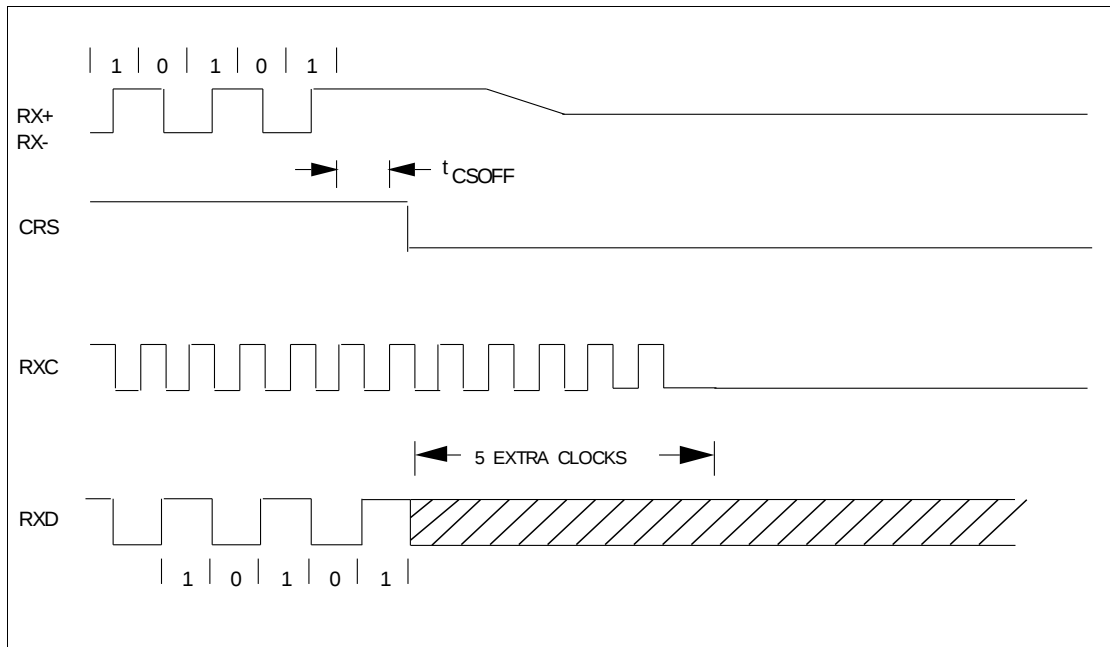
FIGURE 5-7. RECEIVE TIMING - END OF PACKET (LAST BIT = 1)
