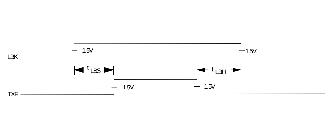
FIGURE 5-11. LOOPBACK TIMING
