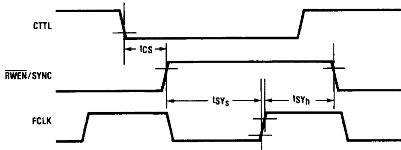
FIGURE 2-11. Synchronization Timing
