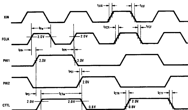
FIGURE 2-3. Clock Signals (b)
