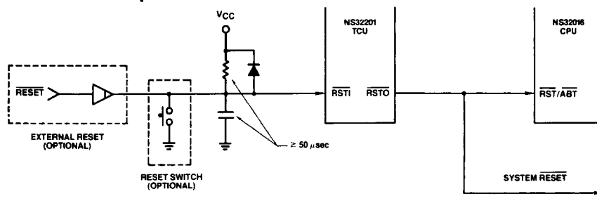
FIGURE 1-3a. Recommended Reset Connections (Non Memory-Managed System)
