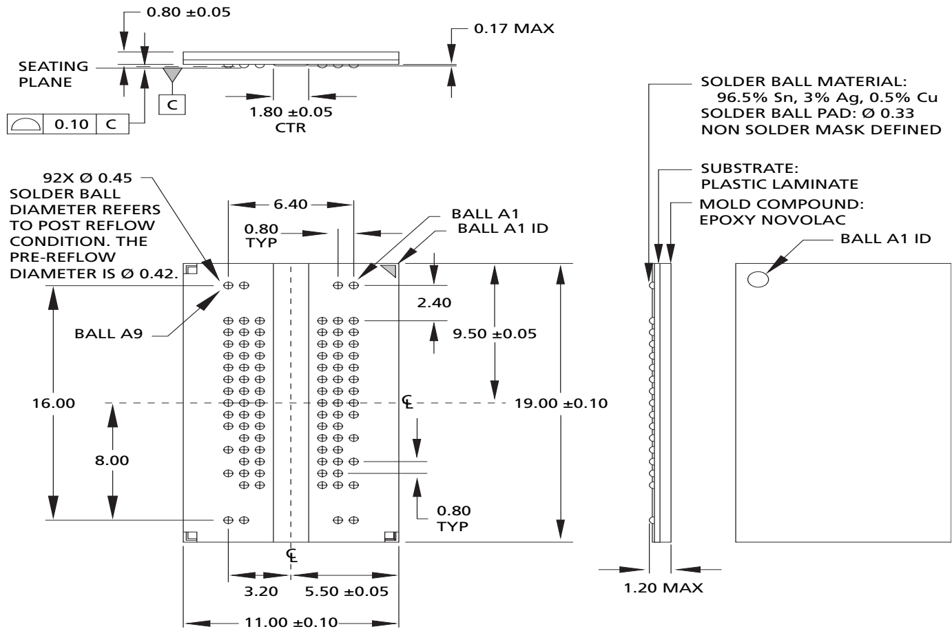
Figure 90: 92-Ball FBGA Package, 11mm x 19mm (x4, x8, x16)
