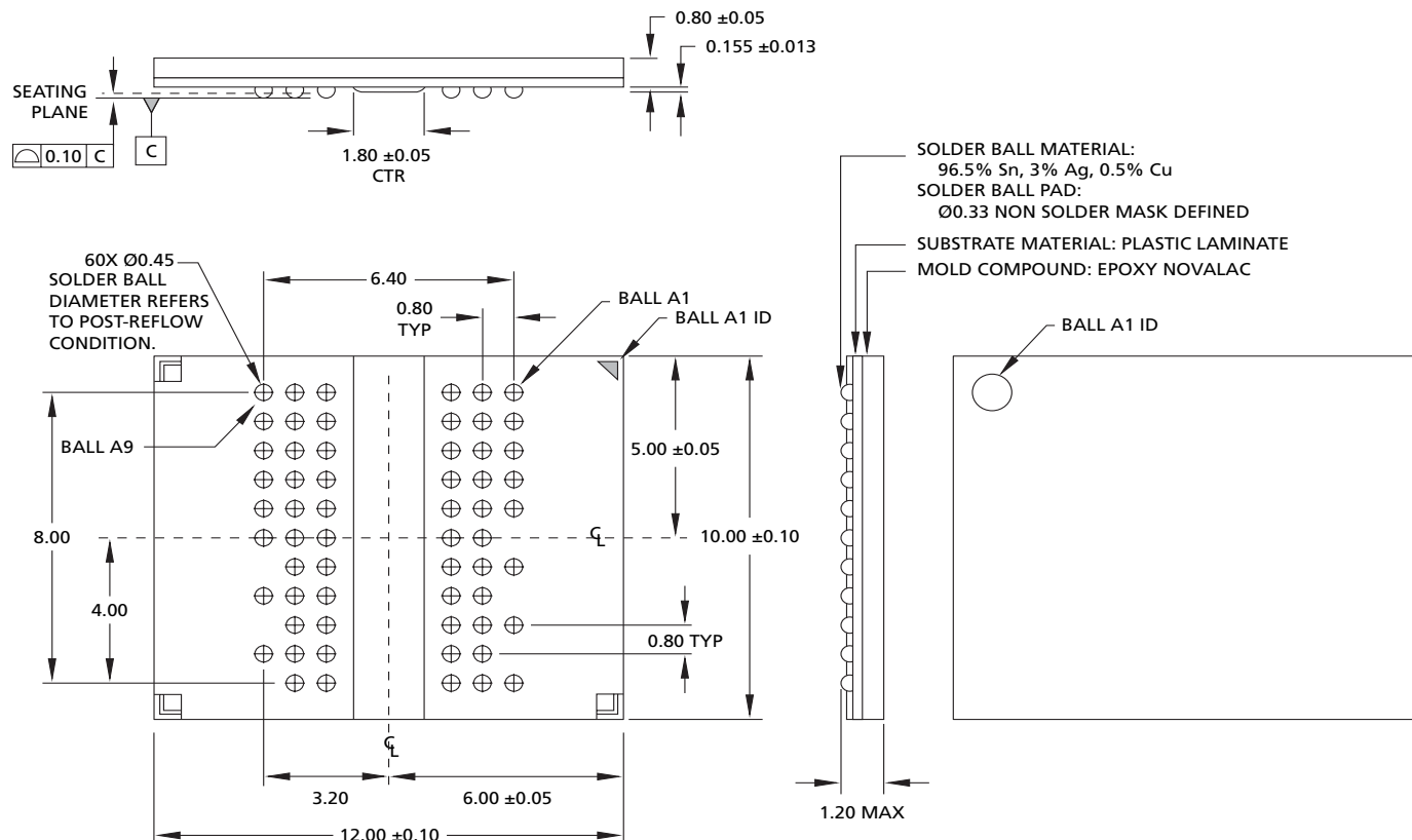
Figure 92: 60-Ball FBGA Package, 12mm x 10mm (x4, x8, x16)
