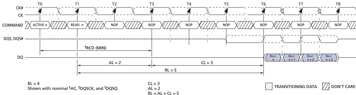
Figure 13: READ Latency
