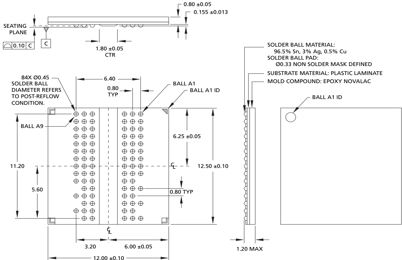
Figure 91: 84-Ball FBGA Package, 12mm x 12.5mm (x4, x8, x16)
