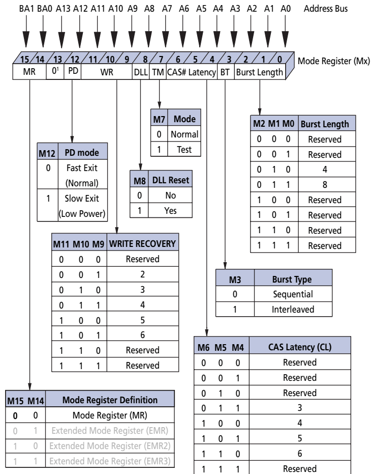
Figure 10: Mode Register (MR) Definition
