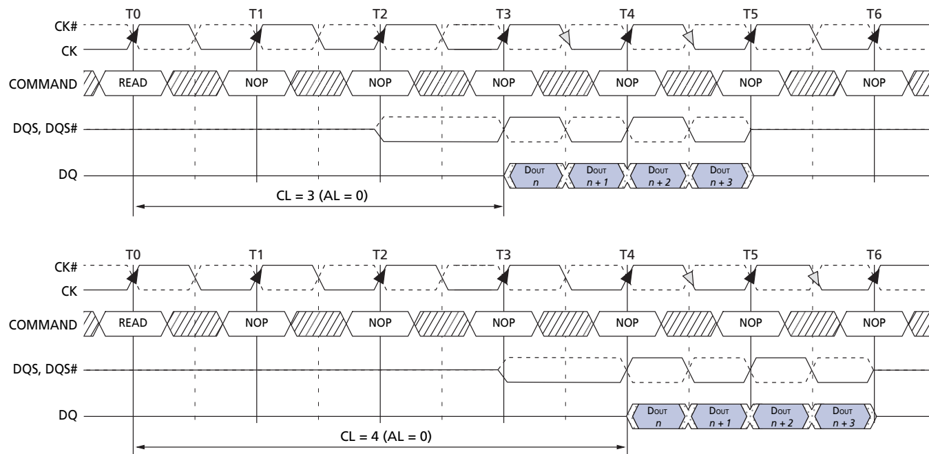
Figure 11: CAS Latency (CL)
