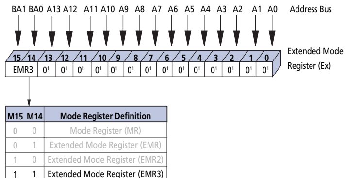
Figure 16: Extended Mode Register 3 (EMR3) Definition
