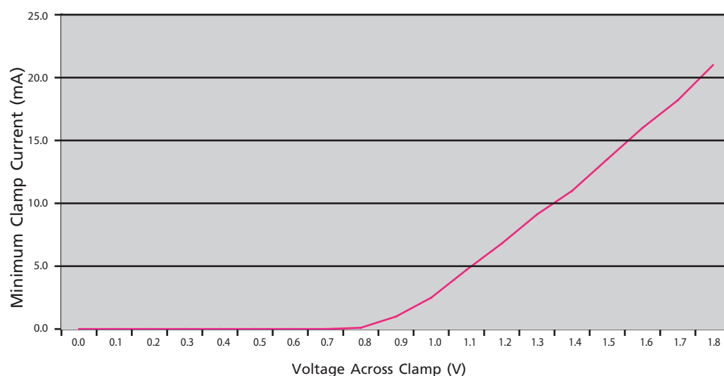
Figure 81: Input Clamp Characteristics
