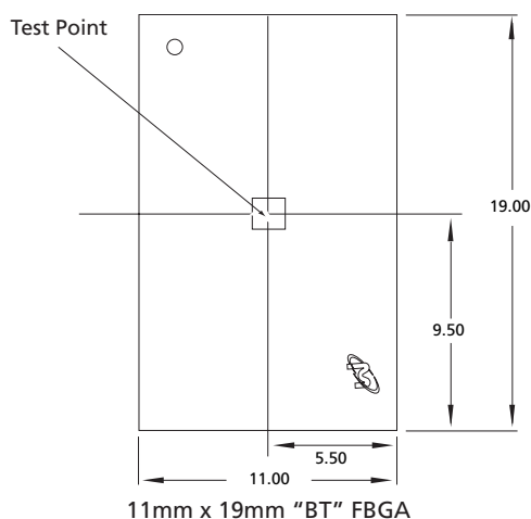
Figure 66: Example Temperature Test Point Location
