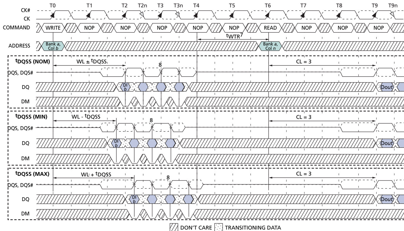
Figure 38: WRITE-To-READ
