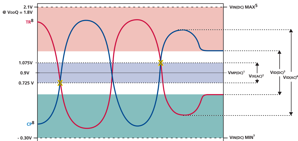
Figure 68: Differential Input Signal Levels
