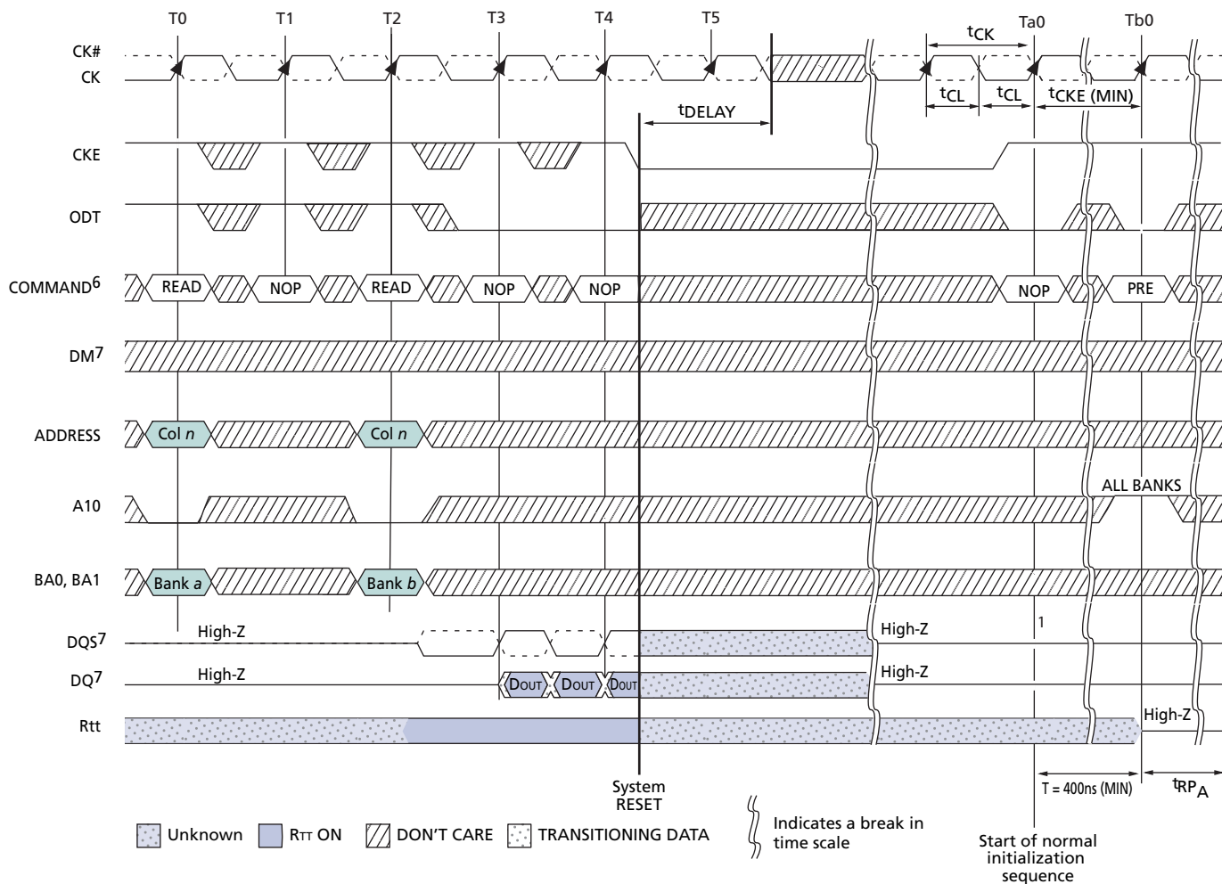
Figure 57: RESET Function
