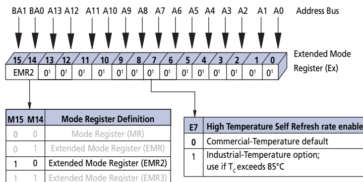
Figure 15: Extended Mode Register 2 (EMR2) Definition
