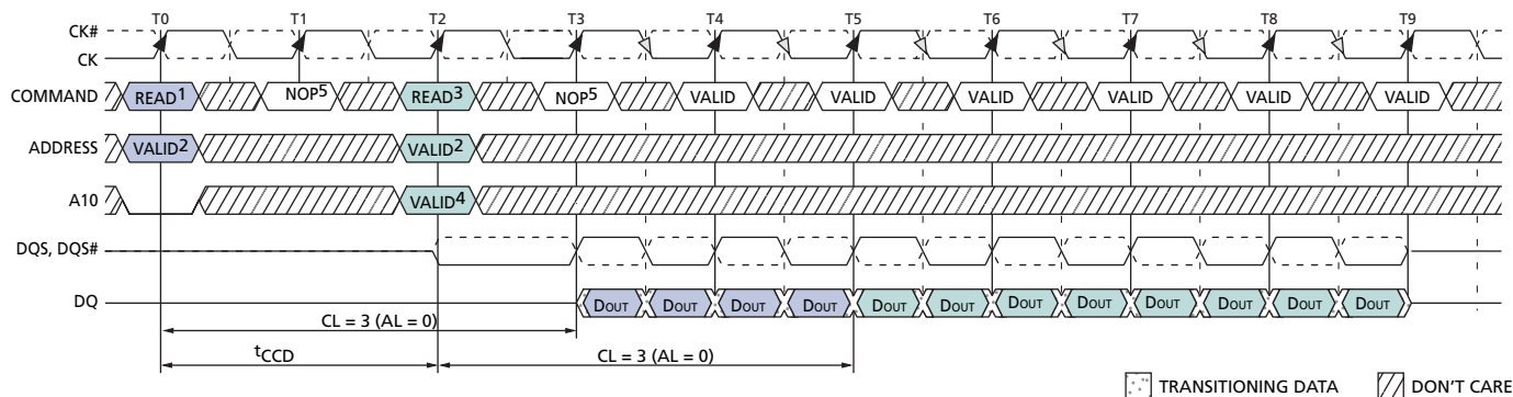
Figure 23: READ Interrupted by READ
