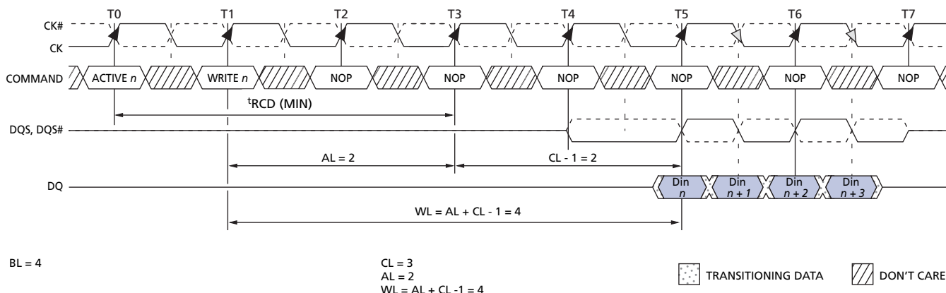
Figure 14: WRITE Latency
