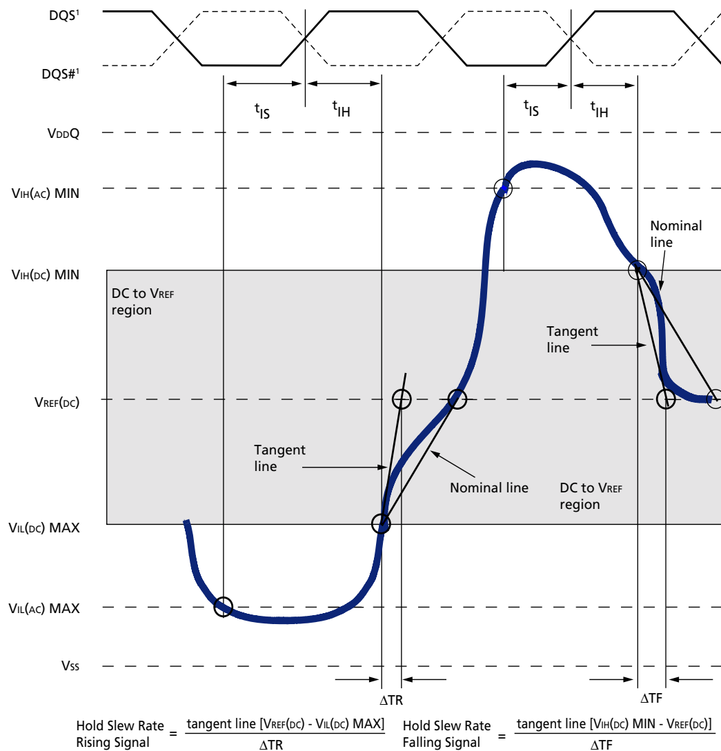
Figure 76: Tangent Line for t_{DH}
