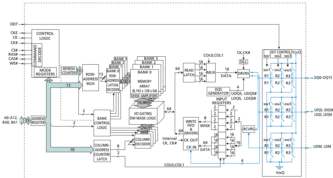
Figure 6: Functional Block Diagram (32 Meg x 16)
