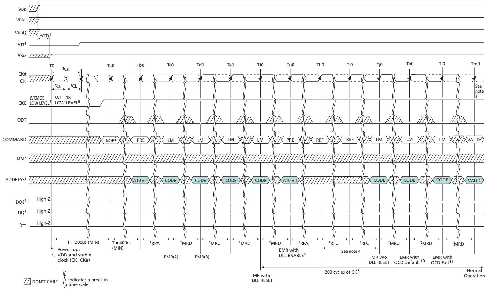
Figure 9: DDR2 Power-Up and Initialization Notes appear on page 24
