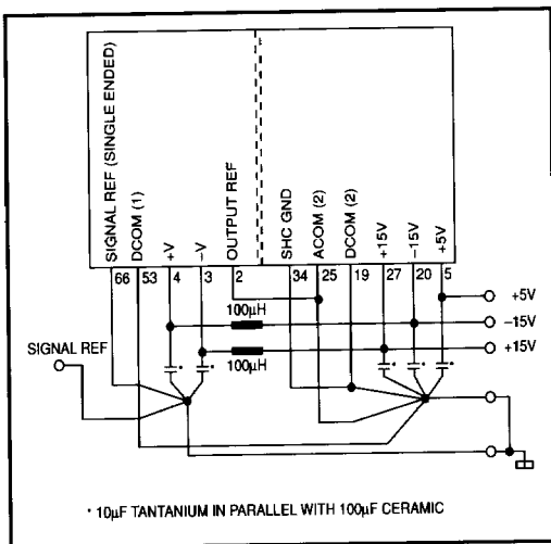
FIGURE 8. Recommended Decoupling of Power Supplies
