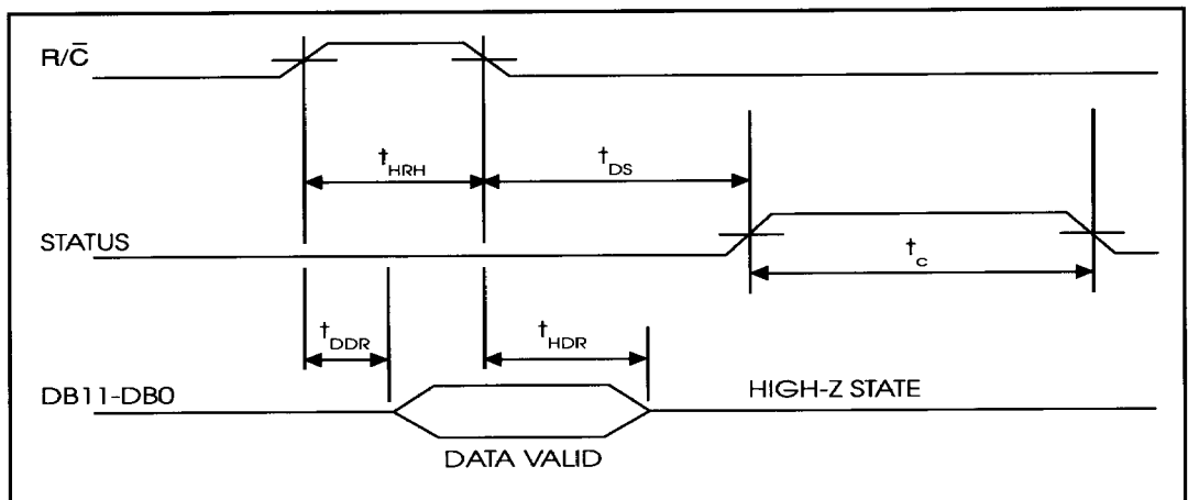
FIGURE 6. High R/C Pulse Conversion Timing
