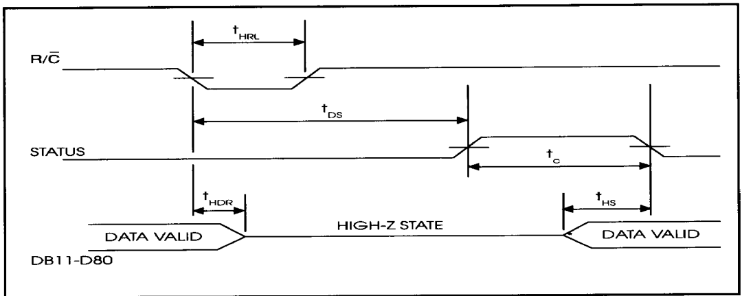
FIGURE 5. Low R/C Pulse Conversion Timing
