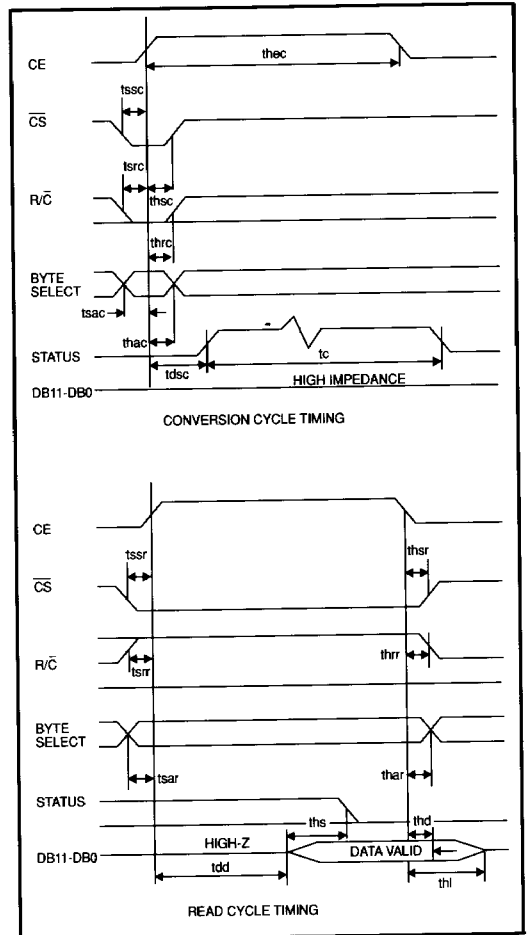
FIGURE 9. Conversion and Read Cycle Timing
