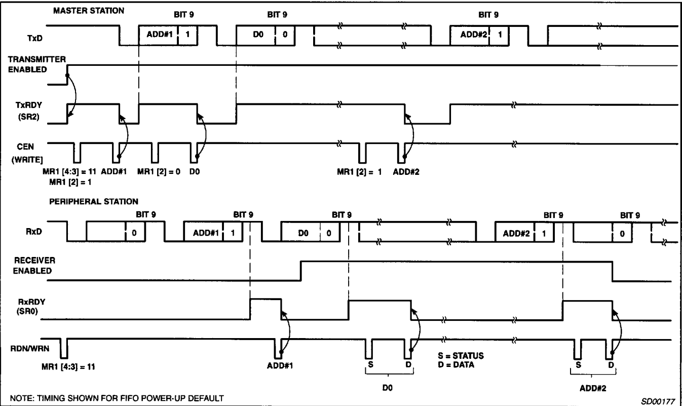
Figure 15. Wake-Up Mode
