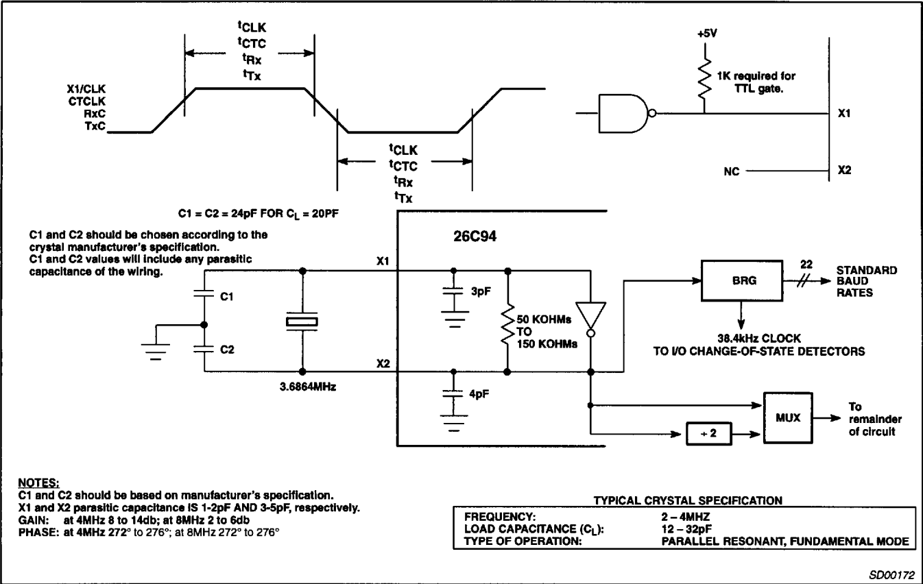
Figure 10. Clock Timing
