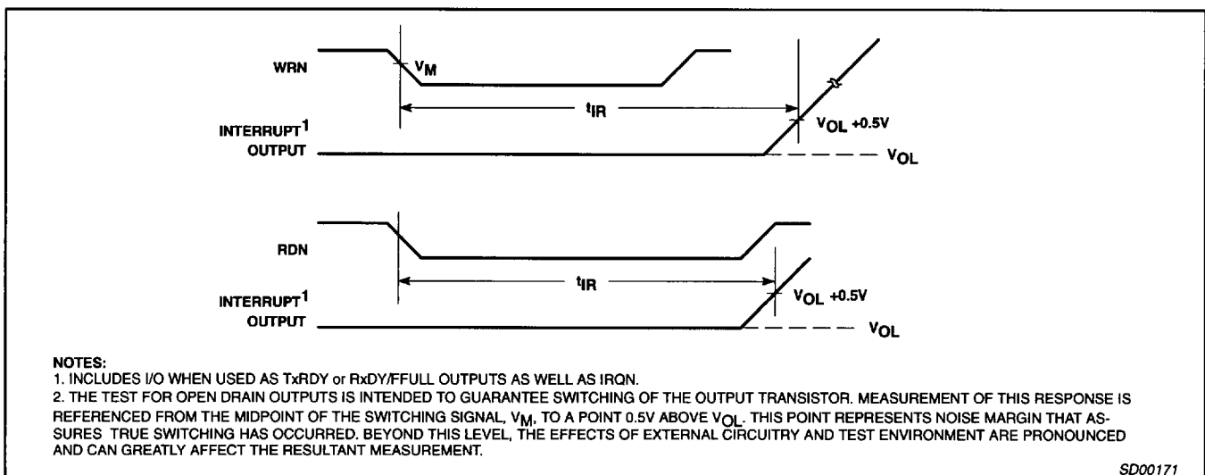
Figure 9. Interrupt Timing
