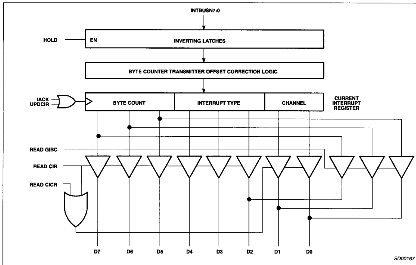
Figure 5. Current Interrupt Register Logic
