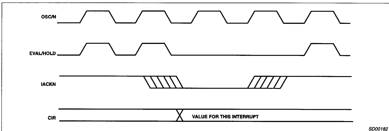
Figure 4. Interrupt Bid Arbitration Timing
