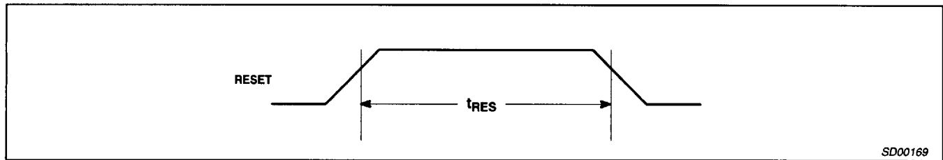
Figure 7. Reset Timing
