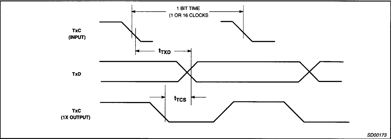
Figure 11. Transit Clock Timing
