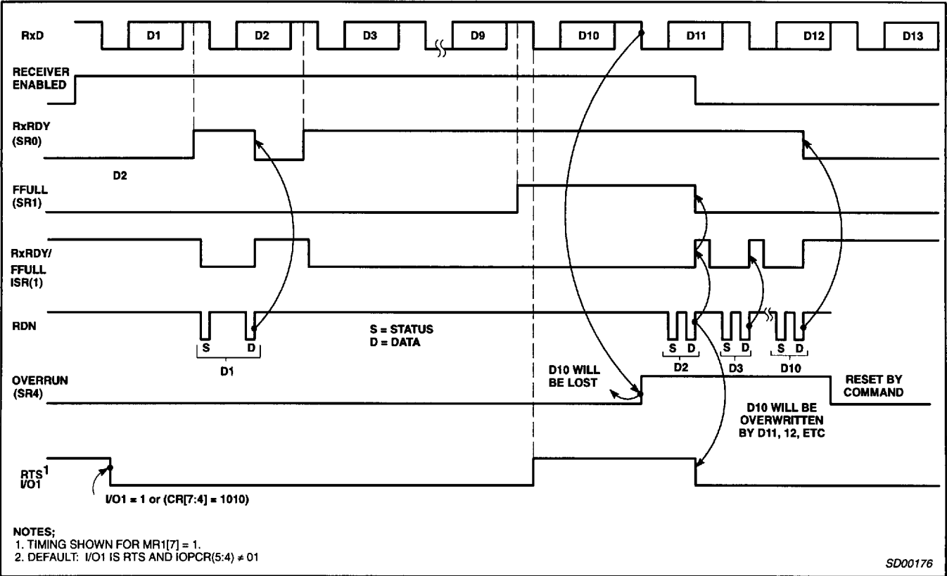
Figure 14. Receiver Data Timing
