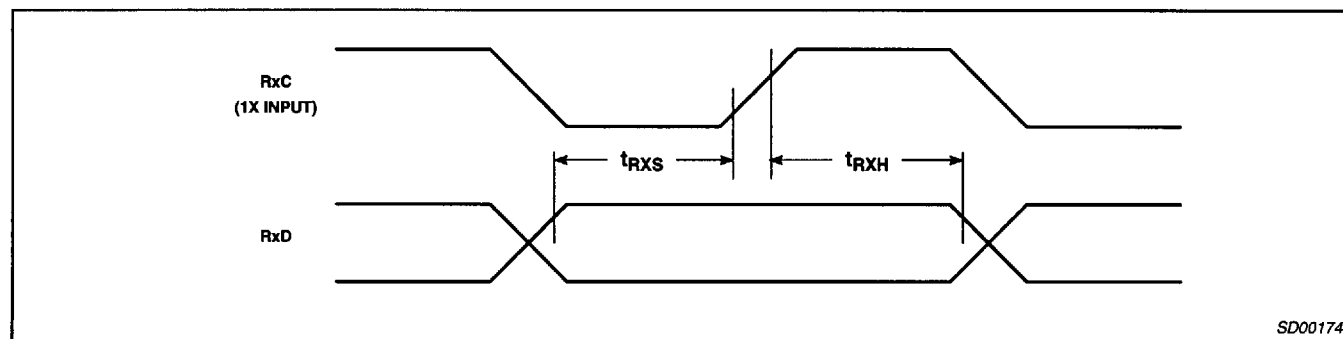
Figure 12. Receive Clock Timing
