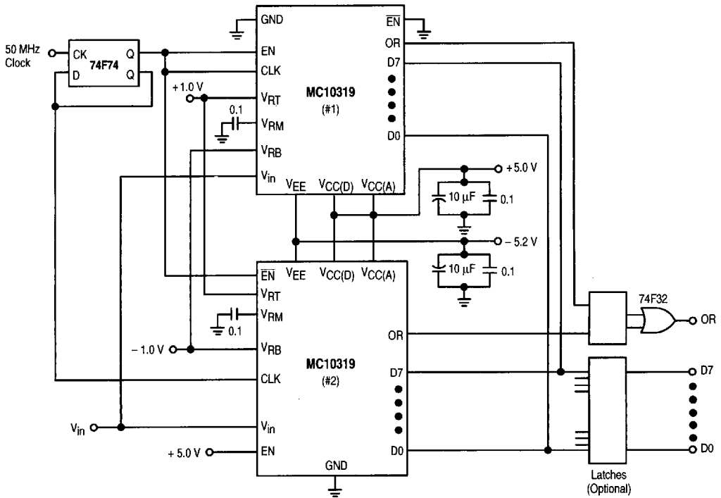
Figure 28. 50 MHz 8-Bit A/D Converter
