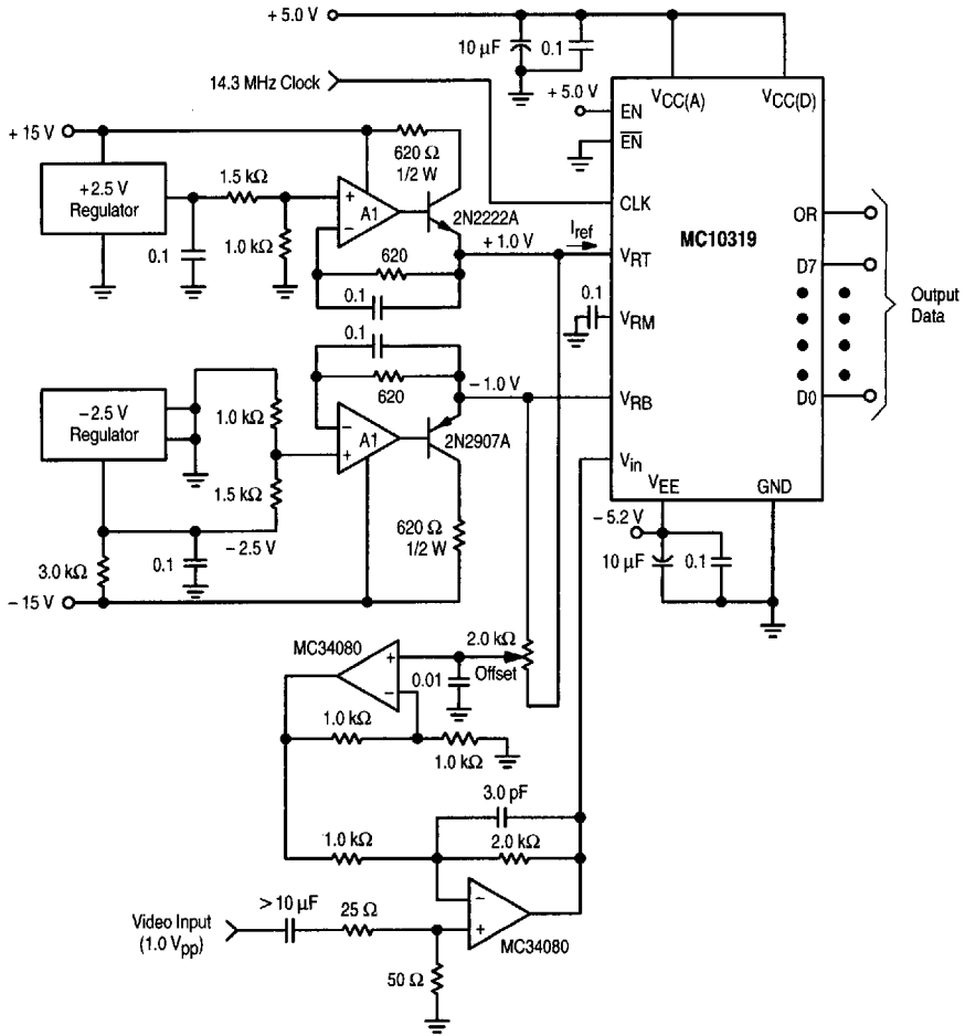
Figure 26. Application Circuit for Digitizing Video
