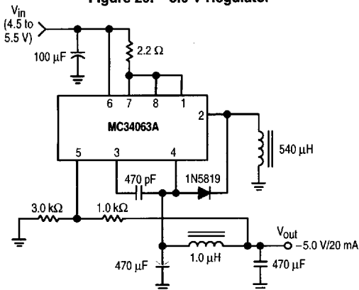
Figure 29. - 5.0 V Regulator
