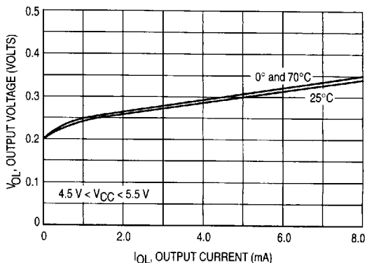
Figure 9. Output Voltage versus Output Current
