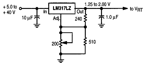
Figure 22. Voltage Source for V_{RT} Pin
