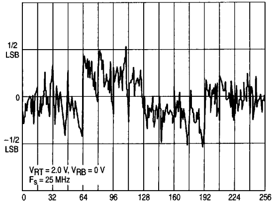
Figure 13. Integral Linearity Error
