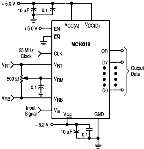
Figure 18. Adjusting V_{RM} for Improved Linearity
