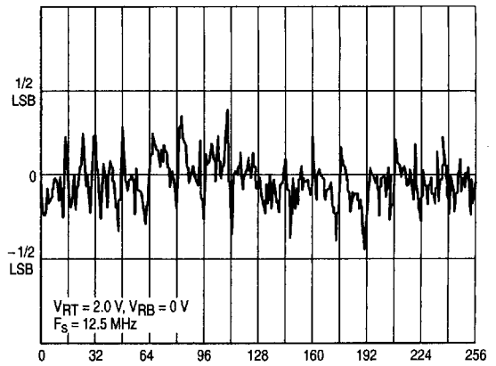
Figure 15. Integral Linearity Error
