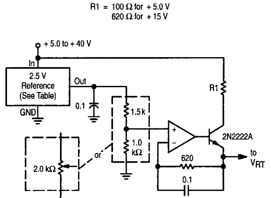
Figure 21. Precision V_{RT} Voltage Source
