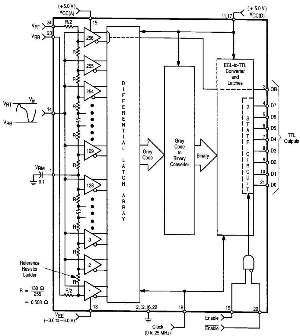
Figure 17. Representative Block Diagram
