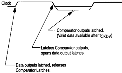
Figure 19. Conversion Sequence
