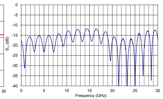
MX-LN-20 Typical S_{11} Curve
