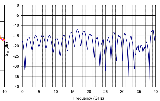
MX-LN-40 Typical S_{11} Curve
