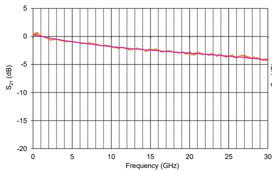
MX-LN-20 Typical S_{21} Curve
