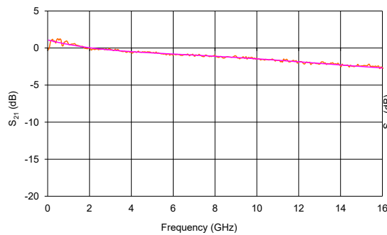
MX-LN-10 Typical S_{21} Curve
