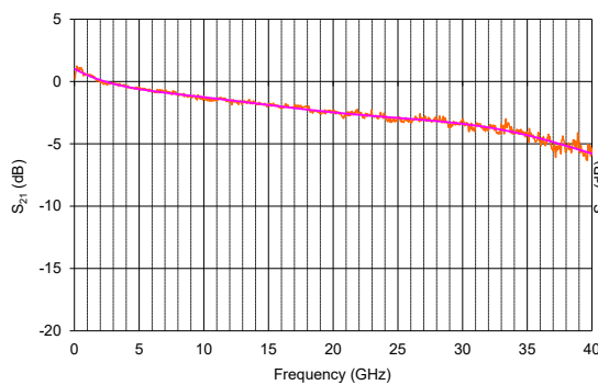
MX-LN-40 Typical S_{21} Curve
