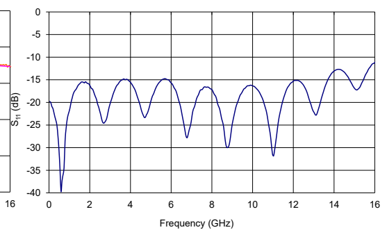
MX-LN-10 Typical S_{11} Curve
