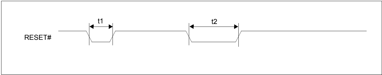
Figure 7-6 S2D13513 RESET# Timing
