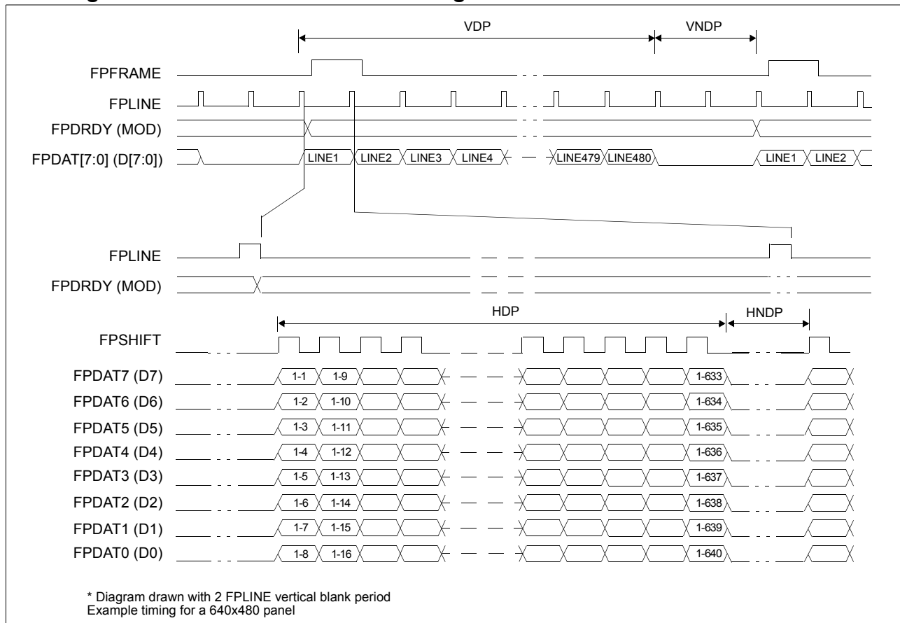
Figure 7-43: Single Monochrome 8-Bit Panel Timing
