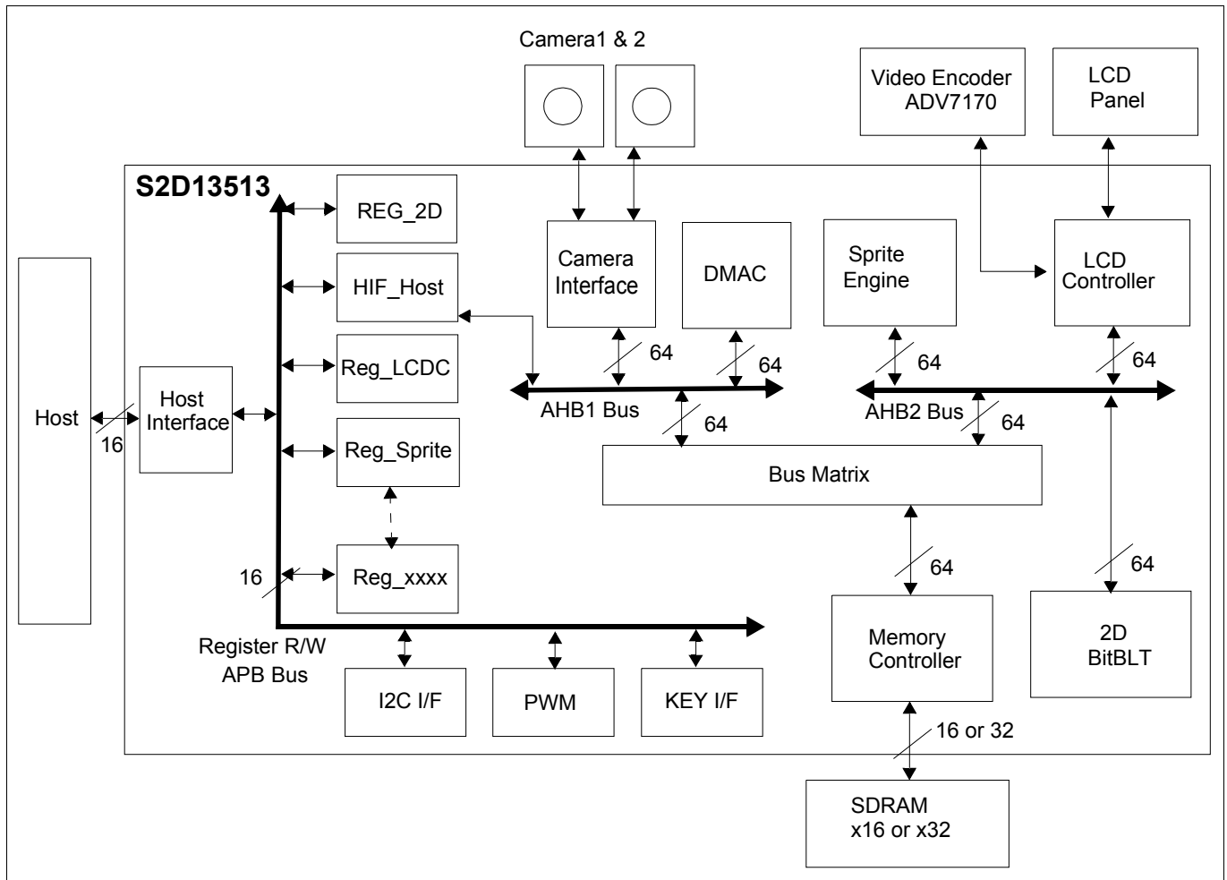
Figure 4-1: Block Diagram
