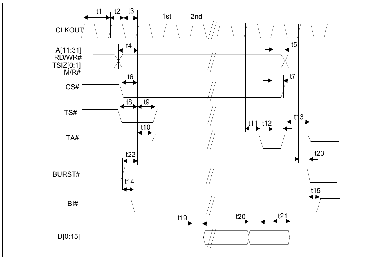
Figure 7-26: Freescale MPC555 Host Interface Read Timing (Non-burst Mode)
