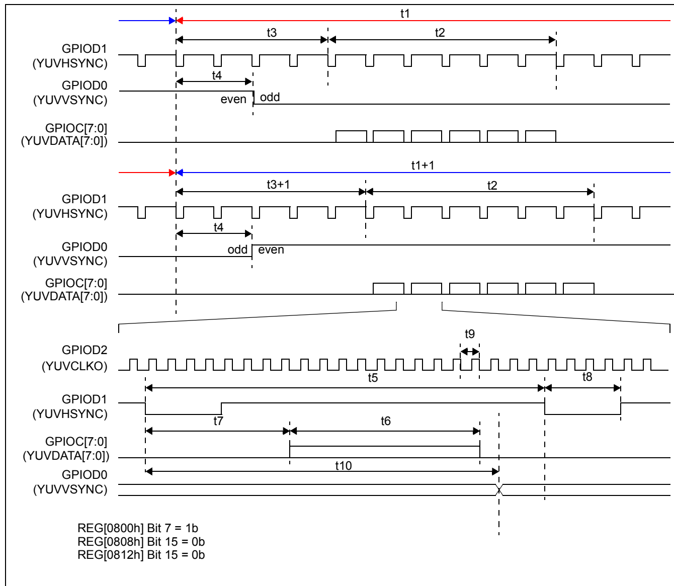
Figure 7-42: YUV Digital Output Interface Timing
