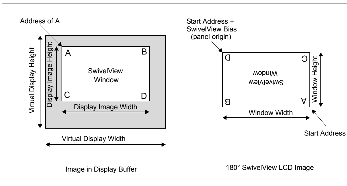
Figure 13-2: Relationship Between Display Buffer Image and LCD Image for 180° SwivelView
