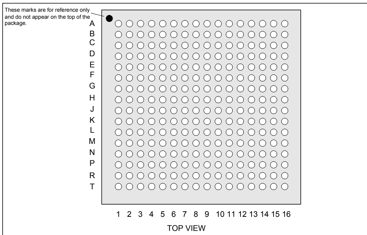
Figure 5-1: PBGA 256-pin Pinout
