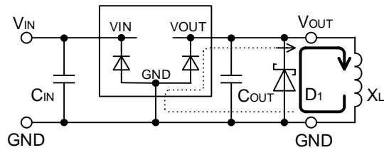
Figure 65. Current Path in Inductive Load (Output: Off)
