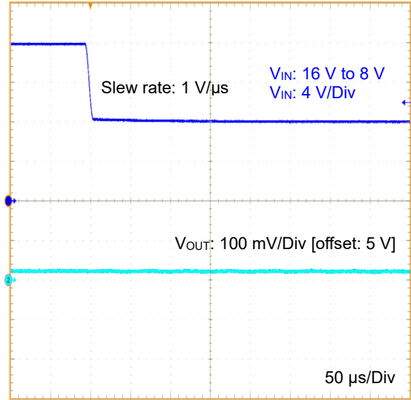
Figure 24. Line Transient 16 V to 8 V (5 V output, I_{OUT} = 0\text{ mA} )
