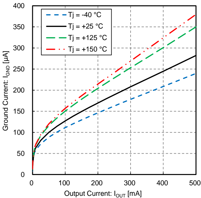
Figure 3. Ground Current vs Output Current (5 V output)
