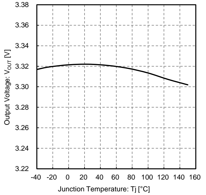
Figure 36. Output Voltage vs Junction Temperature (3.3 V output)
