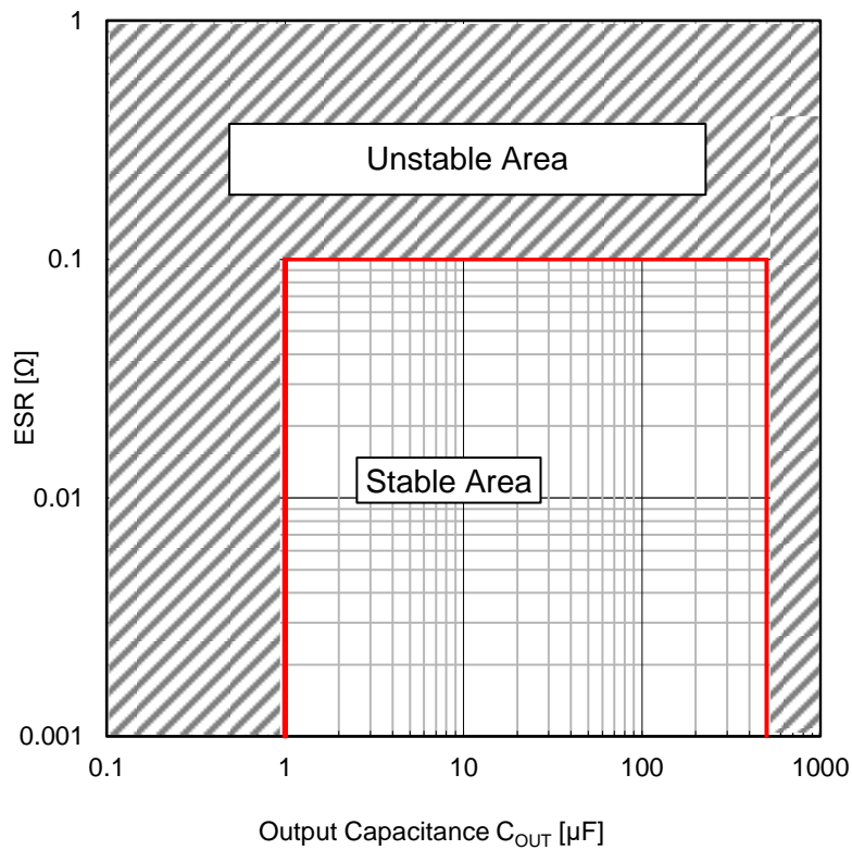
Figure 55. Output Capacitance C_{OUT} , ESR Available Area ( V_{IN} = 4.5\text{ V to }42\text{ V} , V_{OUT} = 1\text{ V}^{(Note 1)} , -40\text{ }^{\circ}\text{C} \leq T_j \leq +150\text{ }^{\circ}\text{C} , I_{OUT} = 0\text{ mA to }500\text{ mA} ) (Note 1) The most strict condition from the stability theory for the control loop of regulator.
