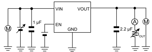
Measurement Setup for Figure 19 to 28, 43 to 52
