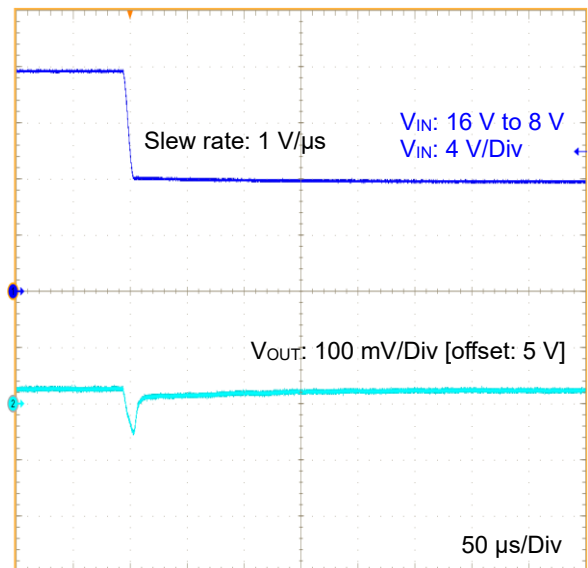
Figure 26. Line Transient 16 V to 8 V (5 V output, I_{OUT} = 500\text{ mA} )
