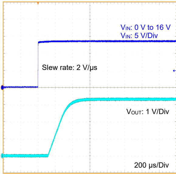
Figure 51. VIN Startup Waveform V_{IN}: 0\text{ V to }16\text{ V} (3.3 V output, I_{OUT} = 0\text{ mA} )
