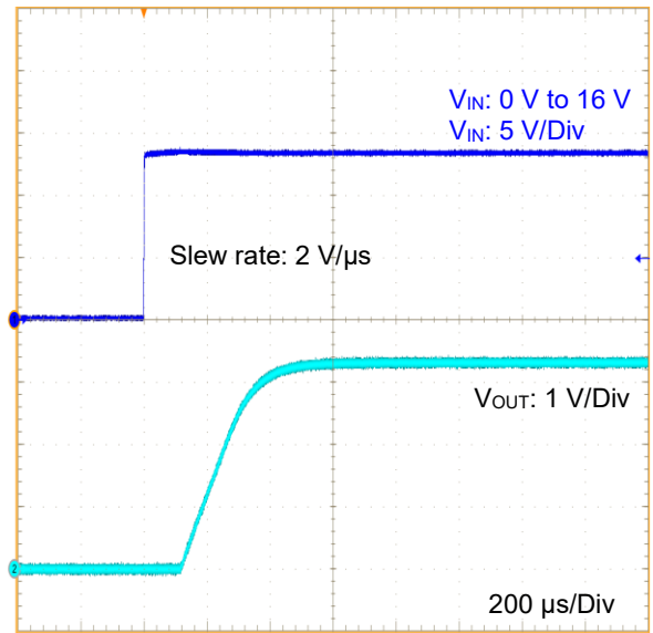
Figure 52. VIN Startup Waveform V_{IN}: 0\text{ V to }16\text{ V} (3.3 V output, I_{OUT} = 500\text{ mA} )
