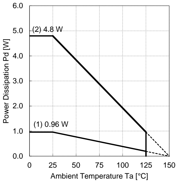
Figure 66. Power Dissipation Graph
