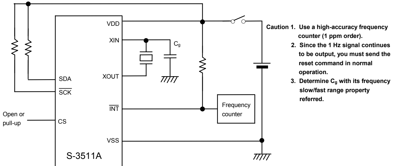
Figure 18 Connection diagram
