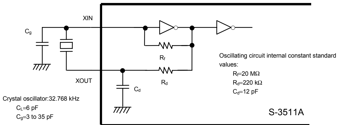
Figure 17 Connection diagram
