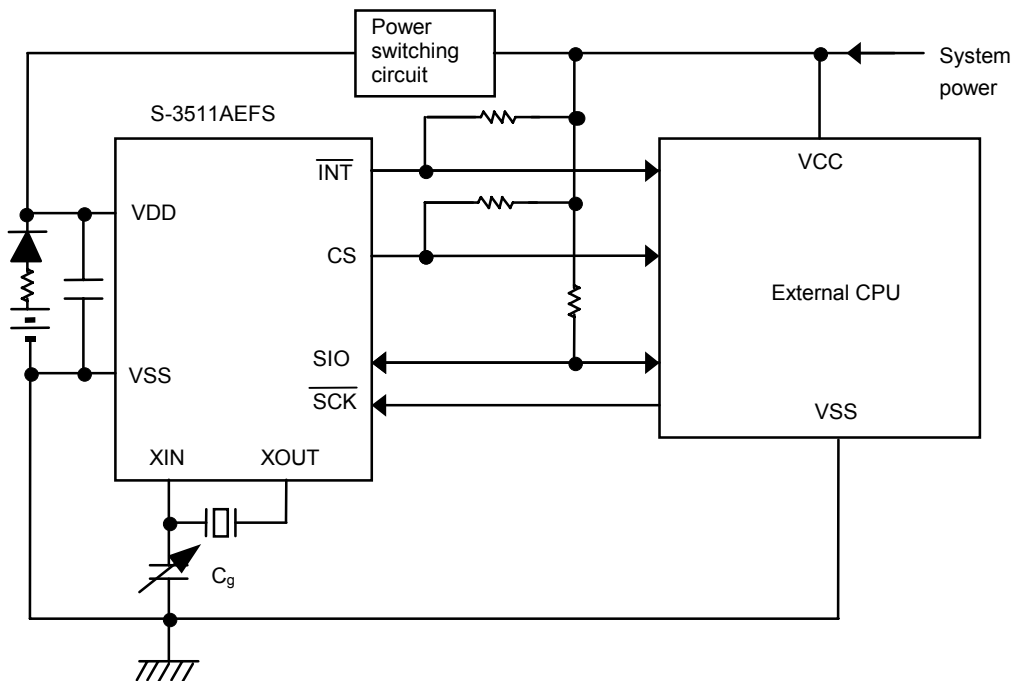
Figure 15 Applied circuit 1
