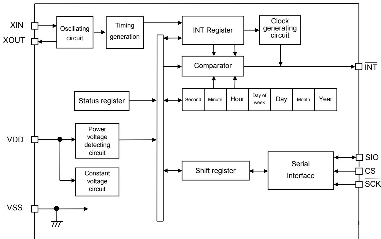
Figure 1 Block diagram
