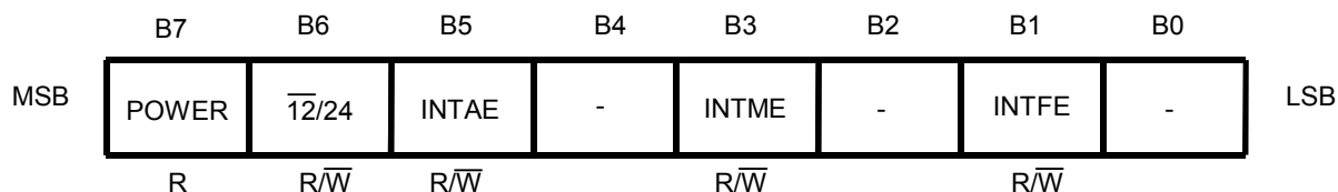
Figure 7 Status register
