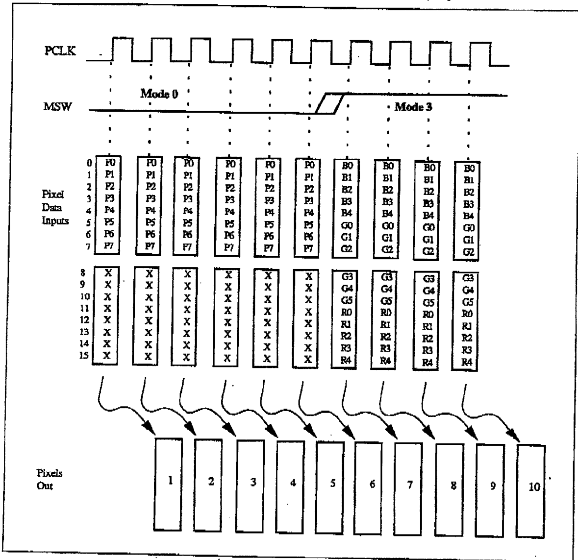
Figure 4: On the fly mode switch from 8bpp to 16bpp (mode 0 changing to mode 3)
