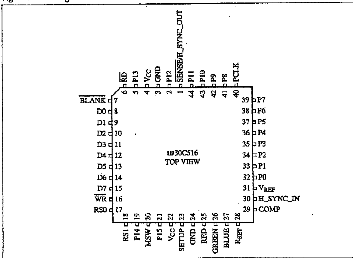
Figure 1: Pin Diagram: W30C516
