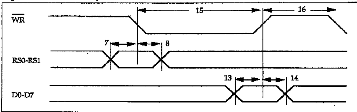
Figure 12: Pixel Input Timing
