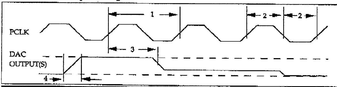
Figure 13: Video Output Timing
