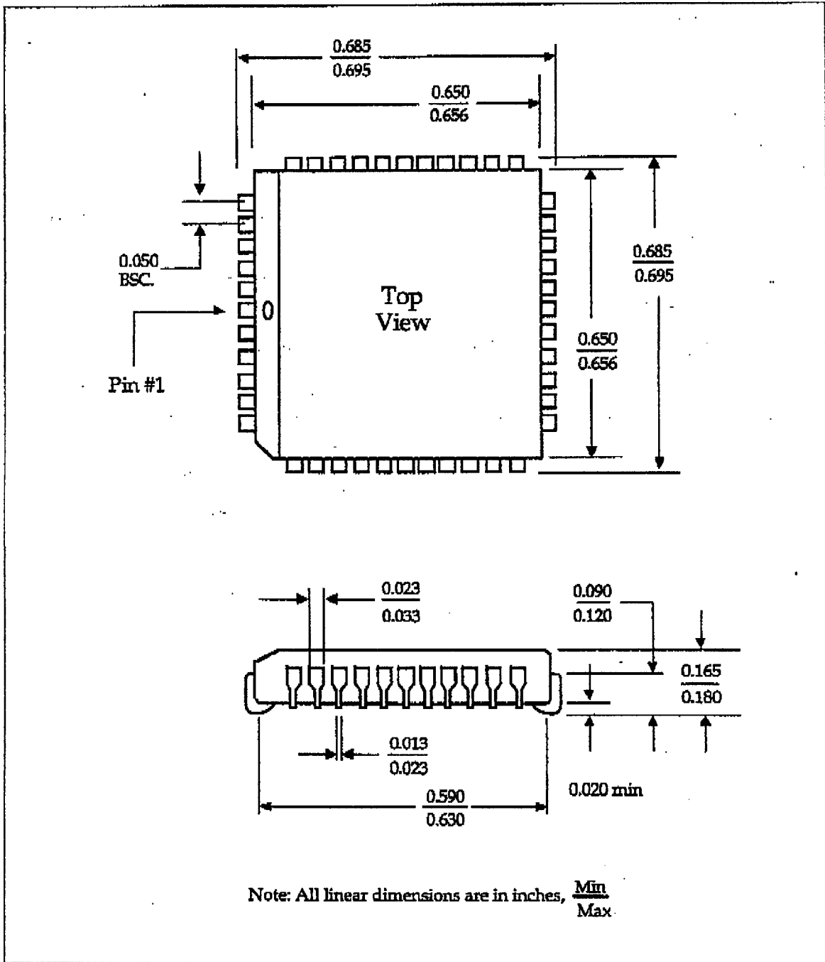
Figure 14: 44 Pin PLCC Package
