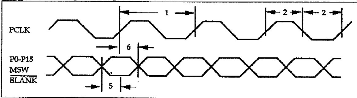
Figure 13: Video Output Timing
