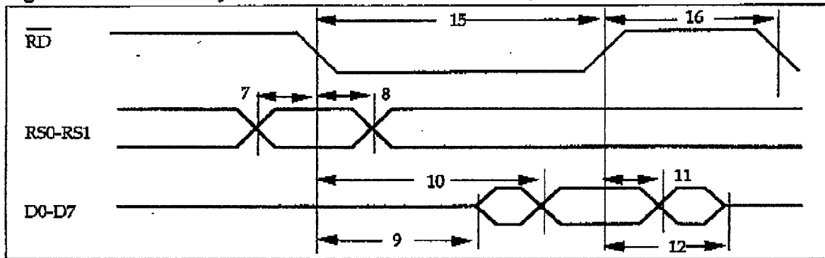
Figure 11: Basic Write Cycle
