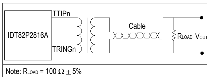
Figure-12 T1 Waveform Template Measurement Circuit
