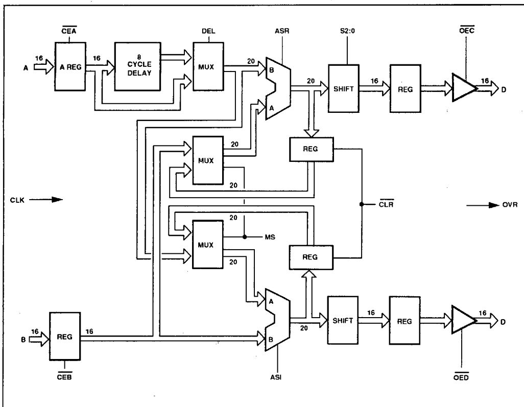
Fig. 3 Block diagram
