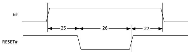
Figure 9. Reset Cycle
