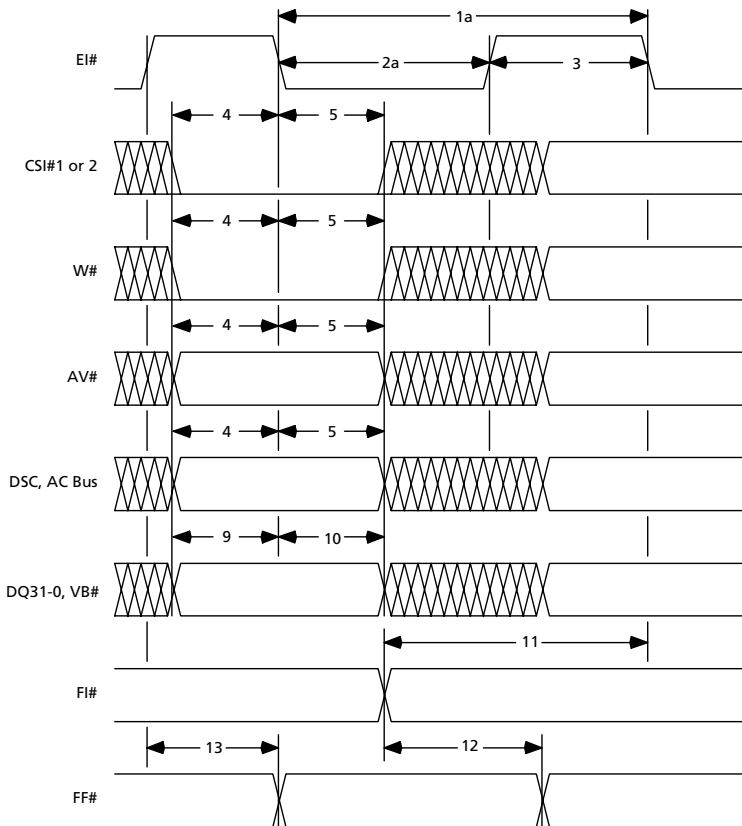
Figure 7. Write Cycle
