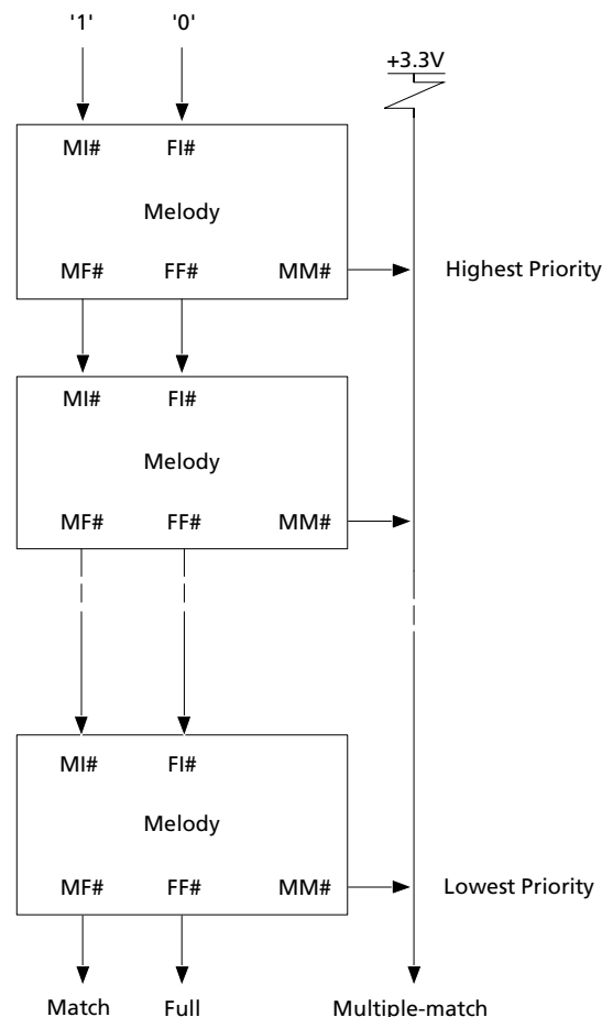
Figure 3. Vertically Cascading Melody TCAMs
