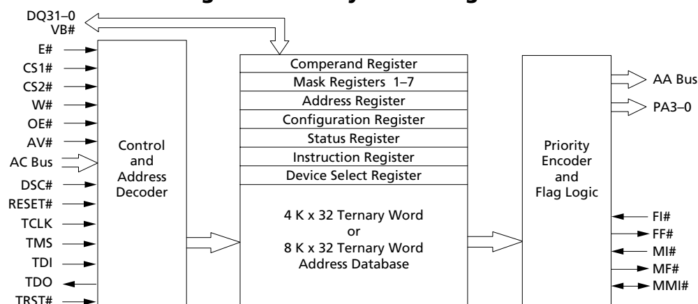
Figure 1. Melody Block Diagram
