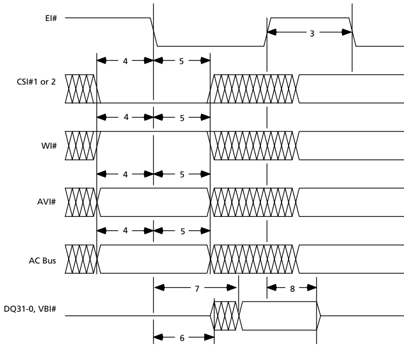
Figure 6. Read Cycle
