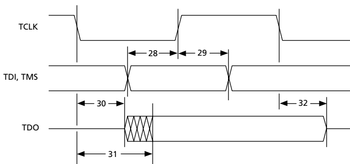
Figure 10. JTAG Test Cycle
