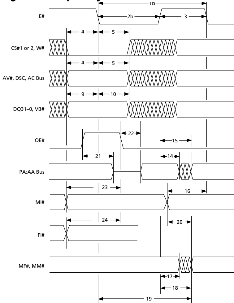
Figure 8. Compare Cycle
