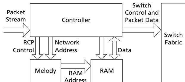
Figure 1. Switch Block Diagram
