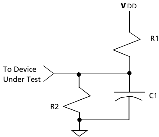
Figure 4. AC Test Load
