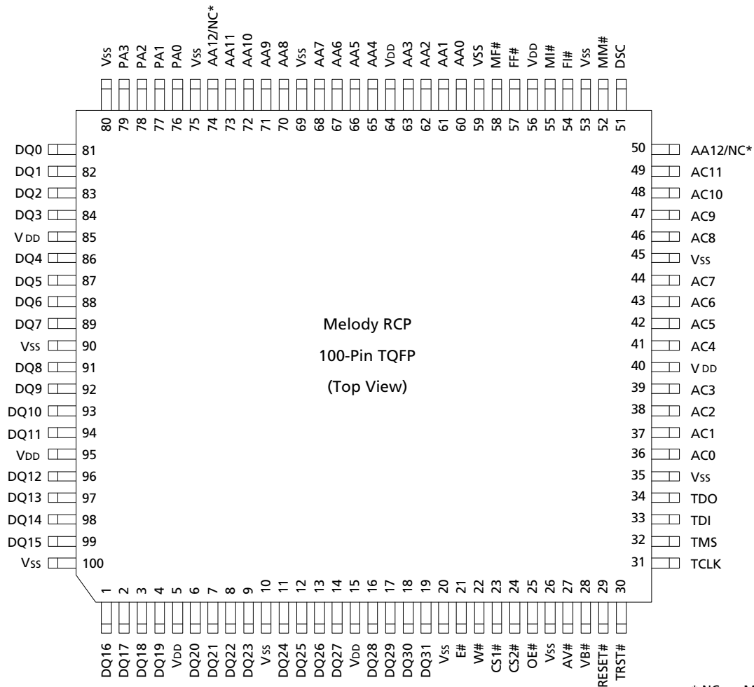
Figure 2. Pin Assignments
