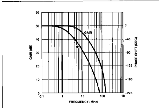
FIGURE 1: Gain-Phase Frequency Response of the Preamplifier
