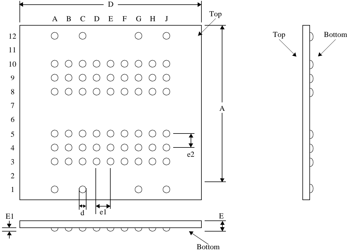
Figure 61: Center-Bonded uBGA Package
