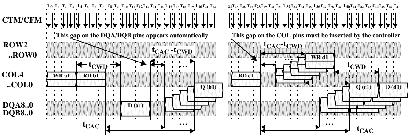
Figure 4: Read (Q) and Write (D) Data Packet - Timing for t_{CAC} = 8, 9, 10, 11, or 12 t_{CYCLE}
