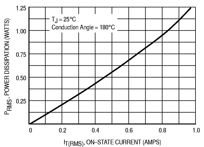
Figure 4. Power Dissipation
