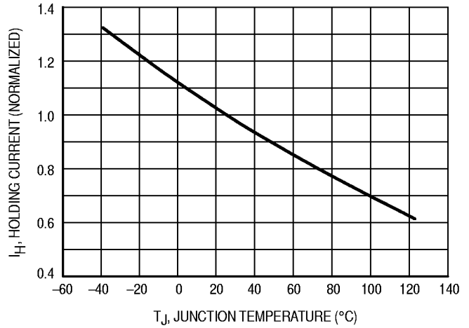
Figure 7. Holding Current
