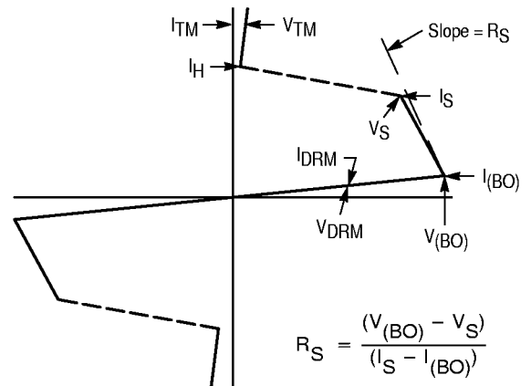
Figure 9. V-I Characteristics
