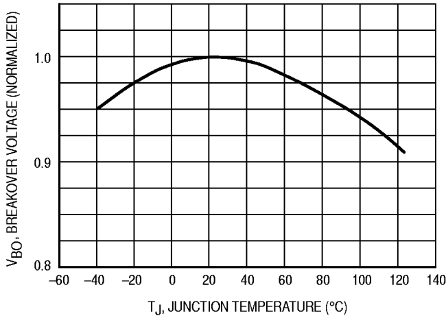
Figure 6. Breakover Voltage
