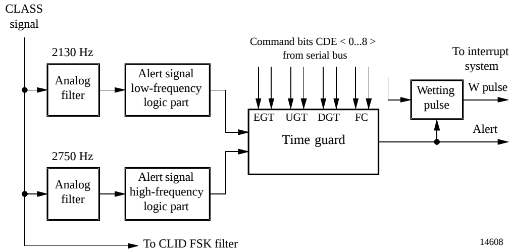
Figure 8. Alert detection
