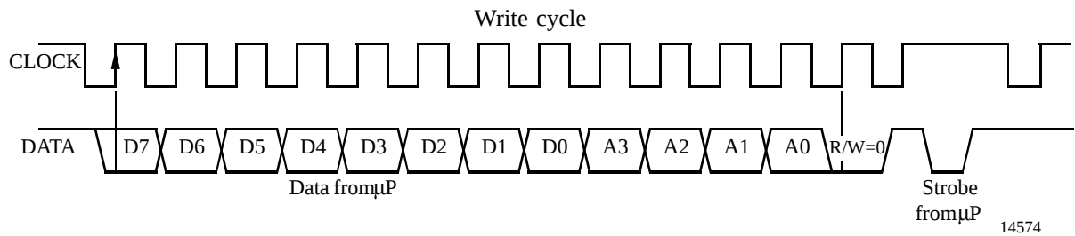
Figure 14. Write cycle
