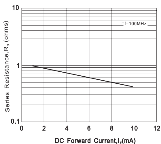
FIG. 4-Series Resistance
