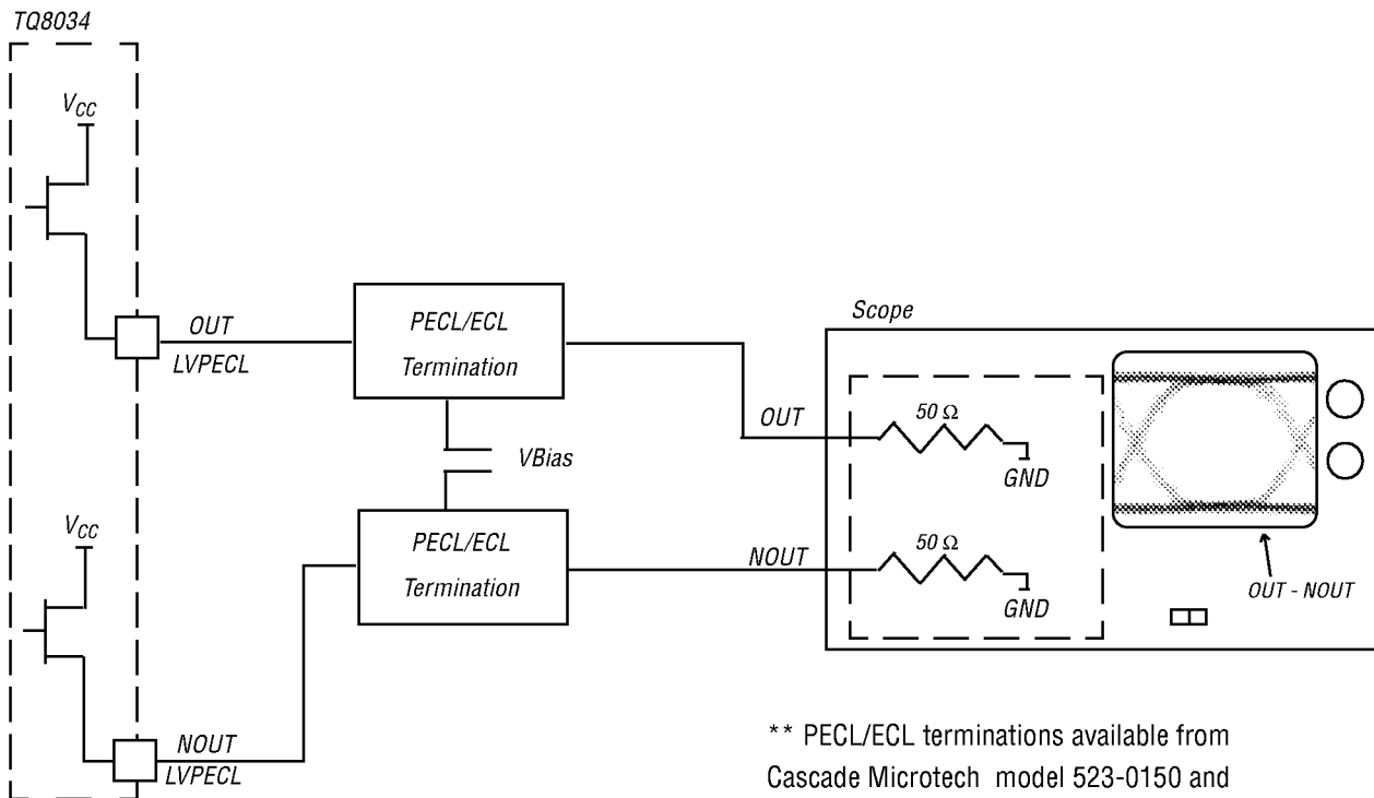
Figure 9. Suggested measurement setup
