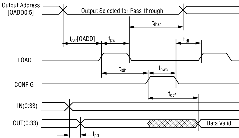
Figure 2. Sequential Configuration (Default Input Address; MODE0 = 0, MODE1 = 1)
