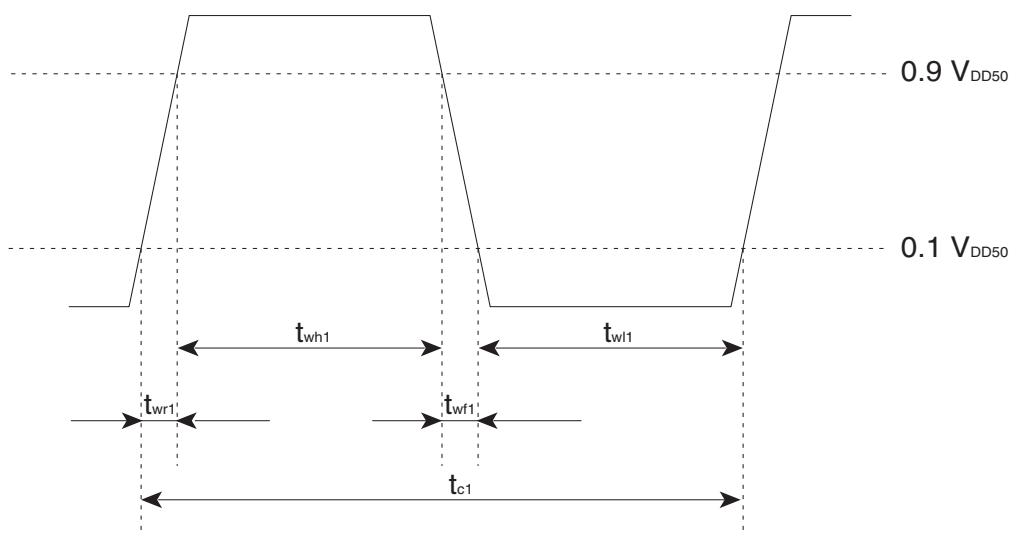
Figure:1.6.3 OSCI Timing Chart
