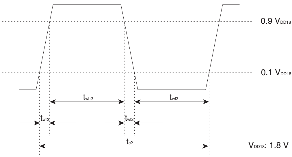
Figure:1.6.4 XI Timing Chart
