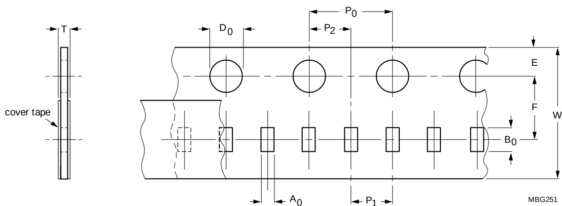
Fig. 15 Paper/PE Tape
