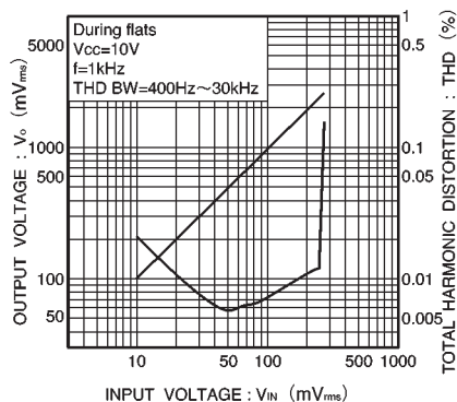
Fig.8 Input/output characteristics
