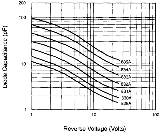
Diode Capacitance
