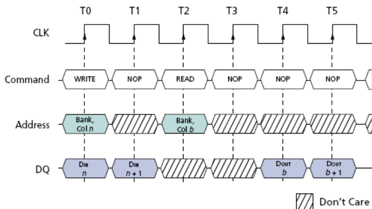
Write-to-Read (CL=2)
