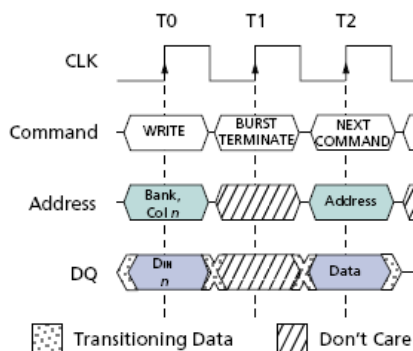
Terminating a WRITE Burst
