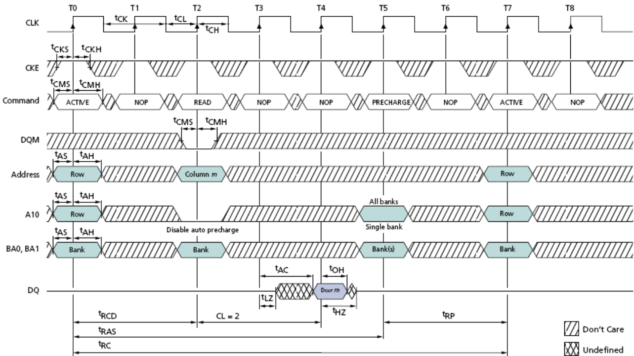
Single READ without Auto Precharge (BL=1 and CL=2)
