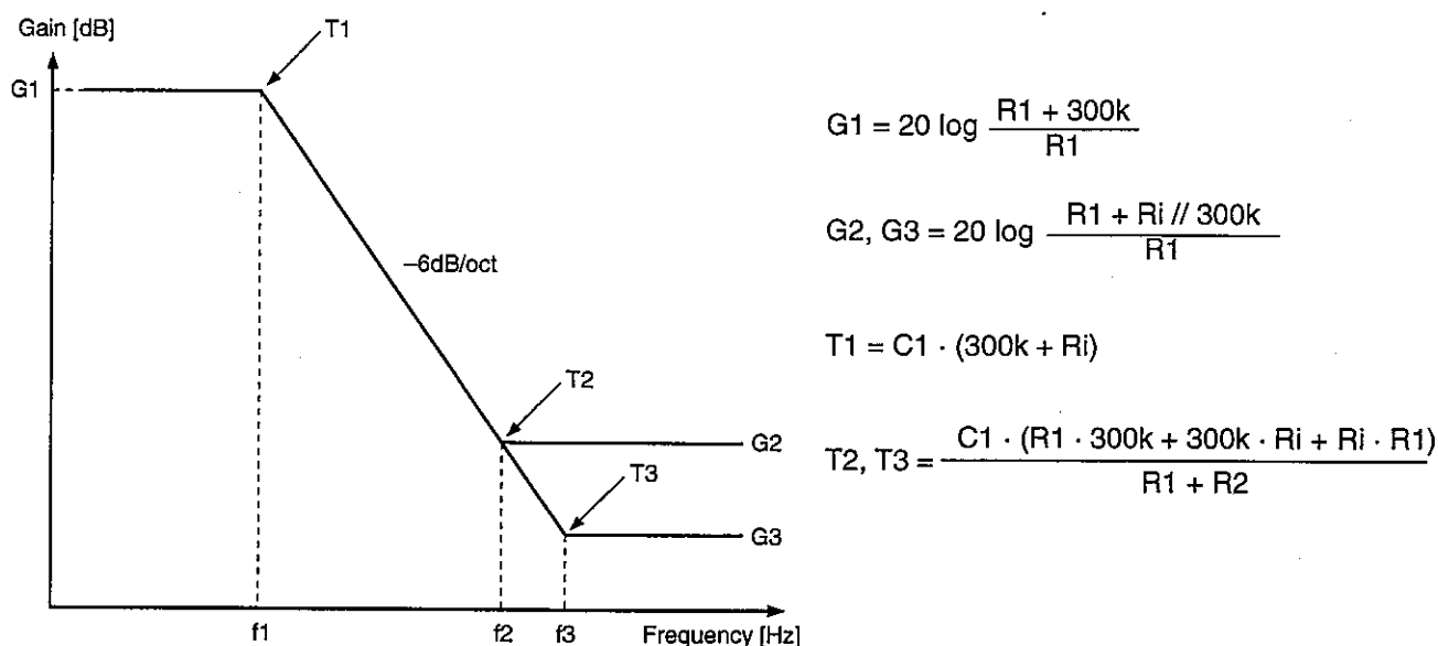
Fig. 4. Playback equalizer amplifier frequency response
