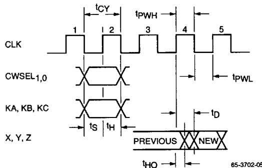
Figure 2. Input/Output Timing
