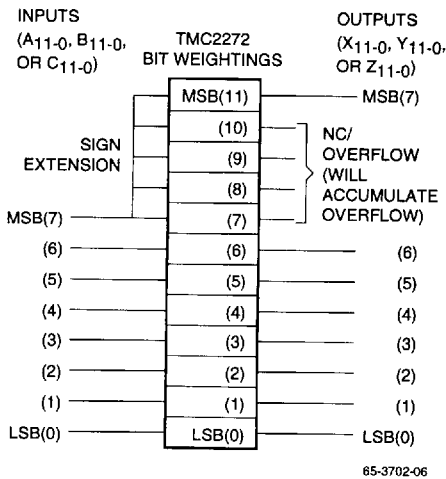
Figure 3. Two's Complement 8-bit Application
