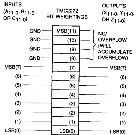
Figure 4. Binary 8-bit Application
