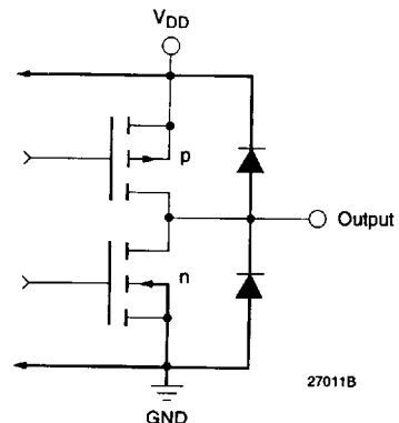
Figure 6. Equivalent Digital Output Circuit
