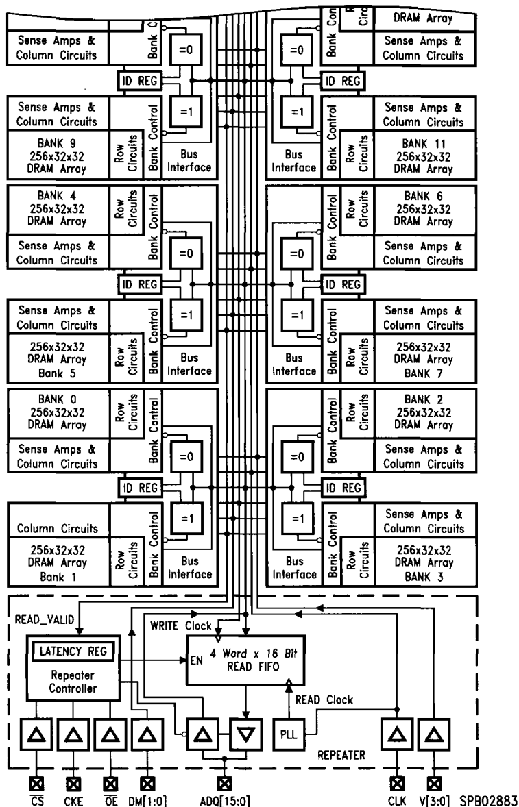
Figure 1 MDRAM Block Diagram
