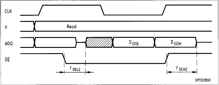
Figure 9 Output Enable Timing
