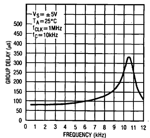
Graph 3. Group Delay
