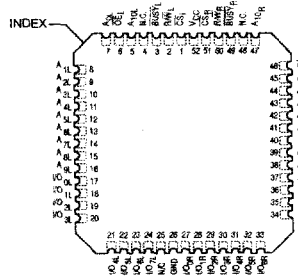
52 PIN PLCC (top view)
