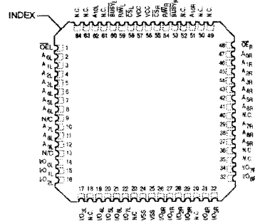
64 PIN VQFP (top view)
