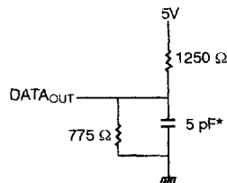
Figure 2. Output load.
