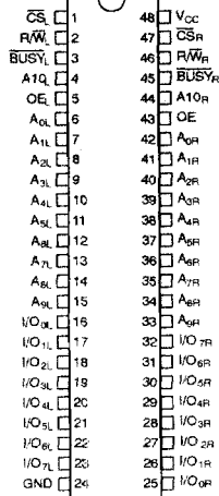
48 PIN DIL (top view), plastic, ceramic 600 mils
