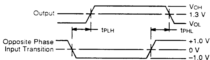
Propagation Delay (Notes 1 and 3)
