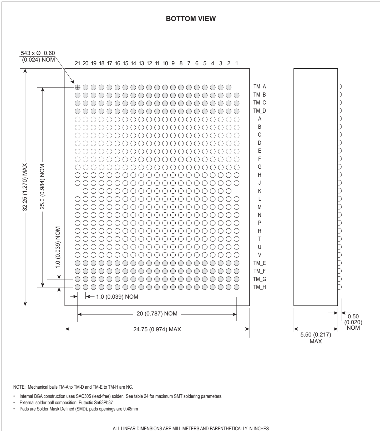
FIGURE 15 – PACKAGE DIMENSION: 543 PLASTIC BALL GRID ARRAY (PBGA) for W3J1G64K-XPBX
