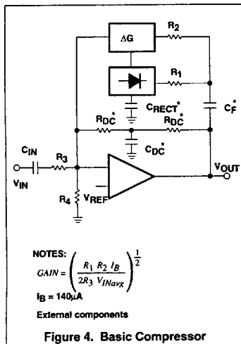
Figure 4. Basic Compressor
