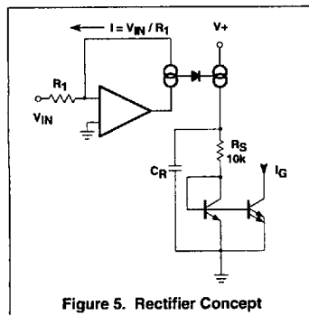
Figure 5. Rectifier Concept
