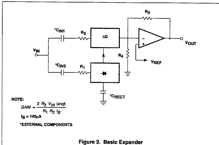
Figure 3. Basic Expander
