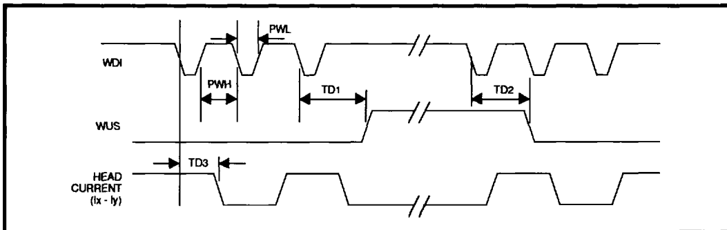
FIGURE 2: Write Mode Timing Diagram (32R2101R)
