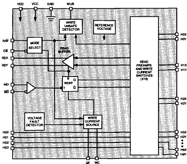
32R2100R BLOCK DIAGRAM
