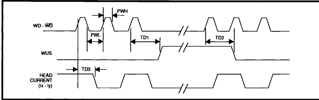
FIGURE 1: Write Mode Timing Diagram (32R2100R)
