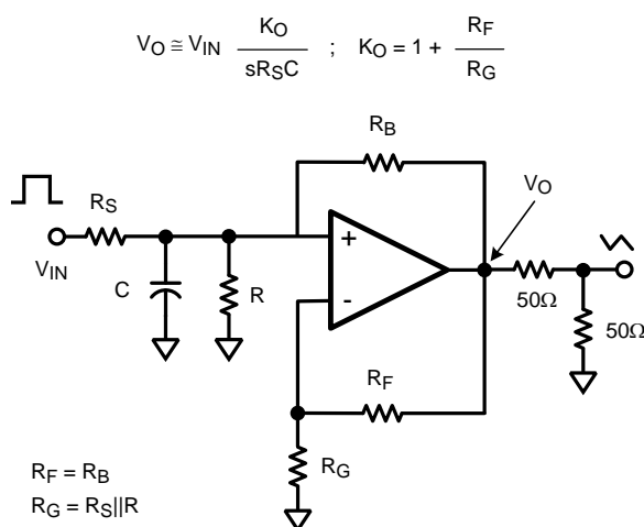
Figure 64. Low-Noise Integrator
