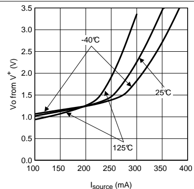
Figure 32. Output Source Current, WSON-8 Package
