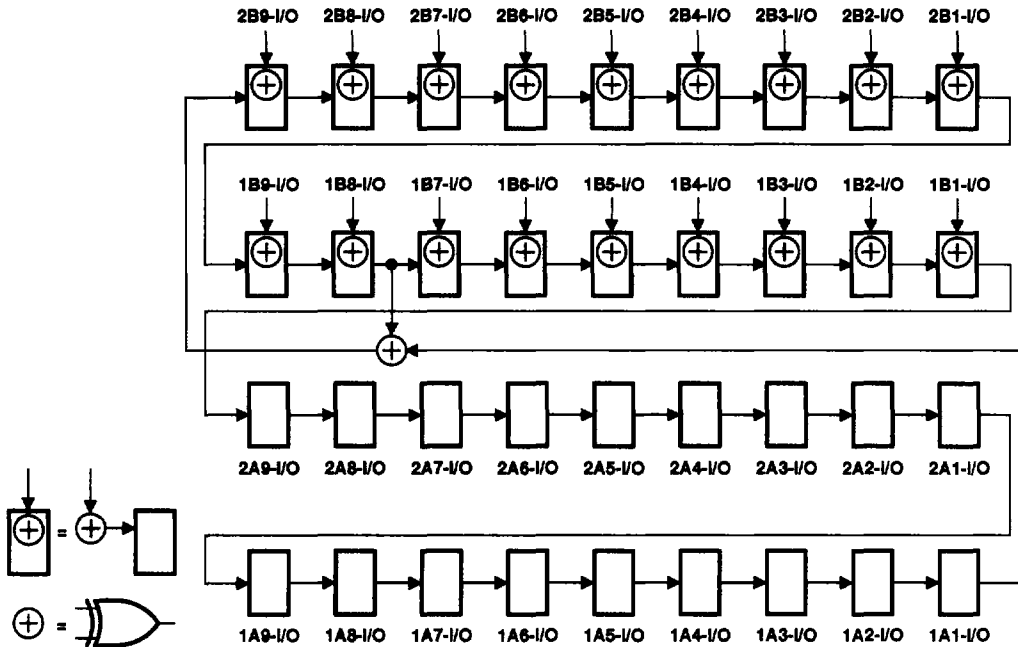
Figure 8. 36-Bit PSA Configuration ( \overline{1OEAB} = \overline{2OEAB} = 1 , \overline{1OEBA} = \overline{2OEBA} = 0 )
