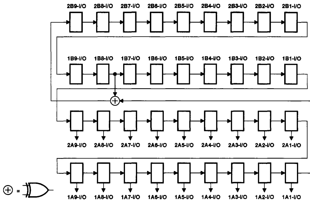
Figure 6. 36-Bit PRPG Configuration ( 1\overline{OEAB} = 2\overline{OEAB} = 1 , 1\overline{OEBA} = 2\overline{OEBA} = 0 )
