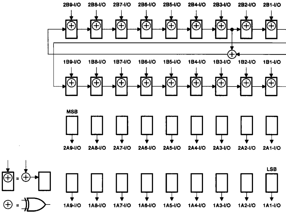
Figure 12. 18-Bit PSA/COUNT Configuration ( \overline{1OEAB} = \overline{2OEAB} = 1 , \overline{1OEBA} = \overline{2OEBA} = 0 )
