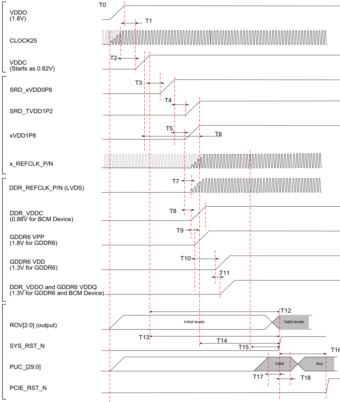
Figure 8: Power-Up Sequence
