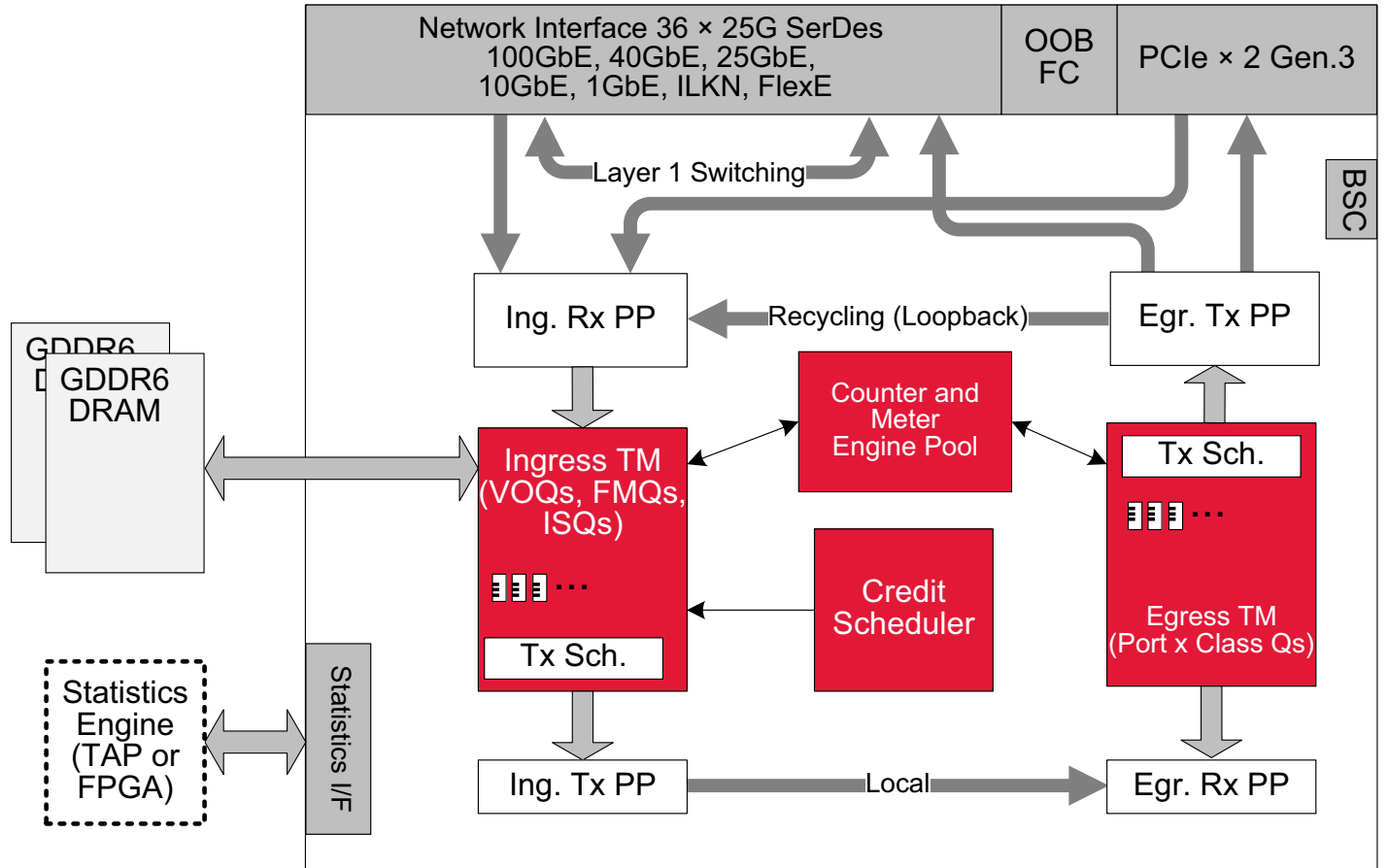
Figure 2: BCM88280 Block Diagram
