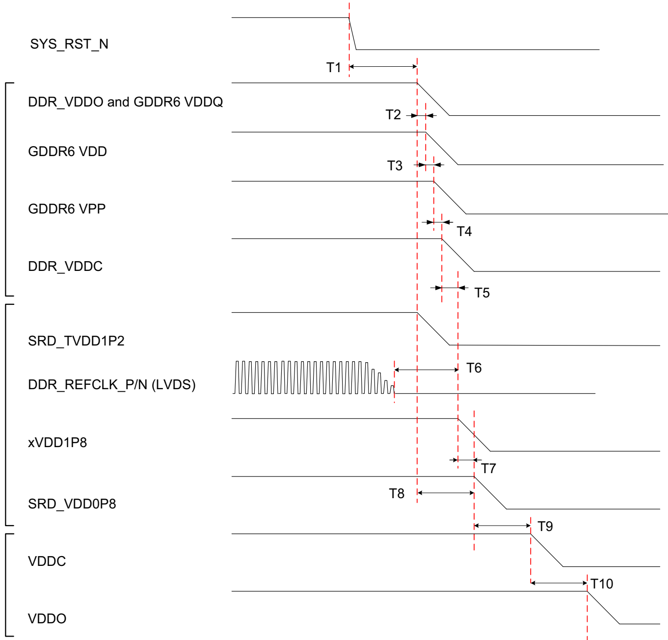
Figure 9: Power-Down Sequence
