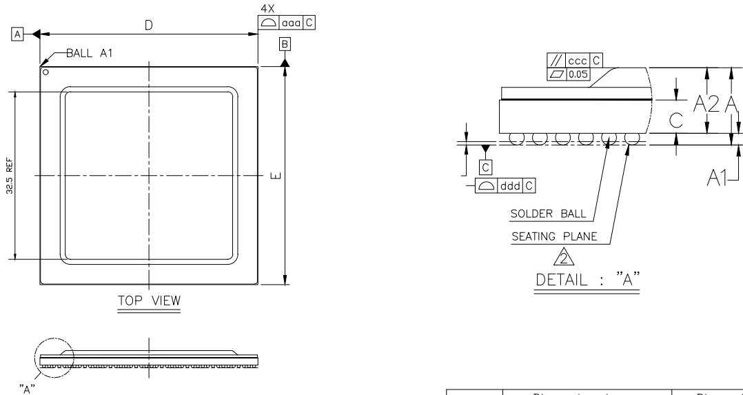
Figure 20: BCM88280 Packaging
