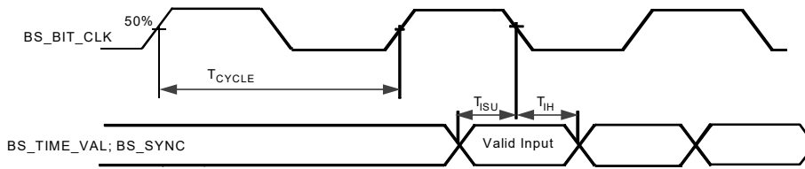
Figure 16: BroadSync Input Timing – timeReceiver Mode
