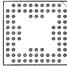
80 PINS PATTERN 1160
