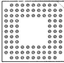
92 PINS PATTERN 1166
