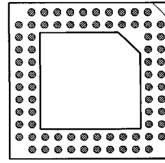
76 PINS PATTERN 1226
