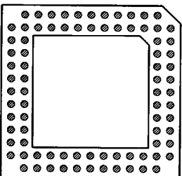
84 PINS PATTERN 1344
