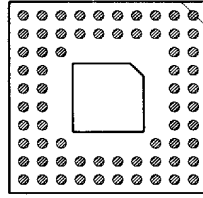
67 PINS PATTERN 1014
