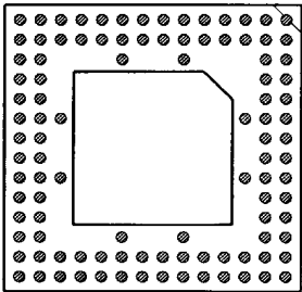
104 PINS PATTERN 1416
