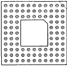
96 PINS PATTERN 1105
