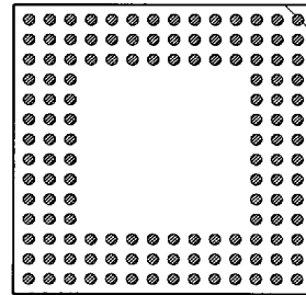
132 PINS PATTERN 1415
