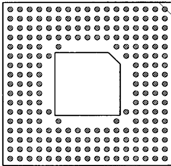
217 PINS PATTERN 1733
