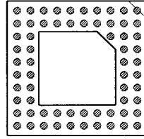
65 PINS PATTERN 1007
