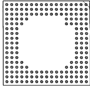
181 PINS PATTERN 1714
