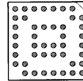
45 PINS PATTERN 0809
