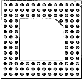
133 PINS PATTERN 1412
