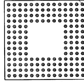
160 PINS PATTERN 1442
