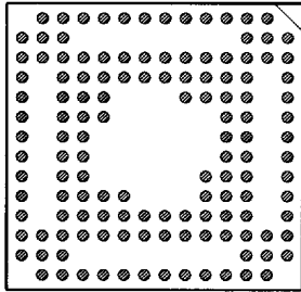
132 PINS PATTERN 1434
