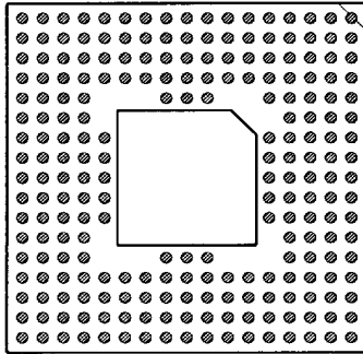
225 PINS PATTERN 1735
