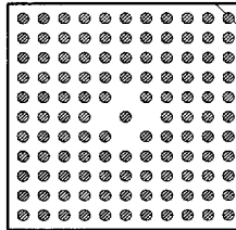
117 PINS PATTERN 1171
