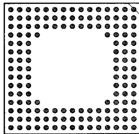
148 PINS PATTERN 1520
