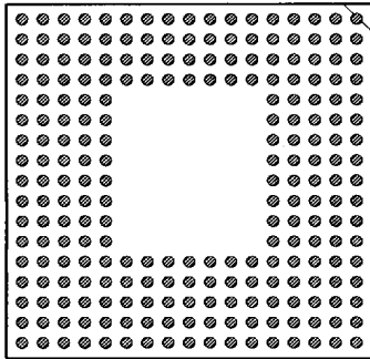
233 PINS PATTERN 1736
