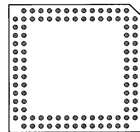
100 PINS PATTERN 1530
