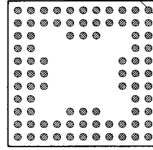
84 PINS PATTERN 1110
