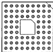
72 PINS PATTERN 0903
