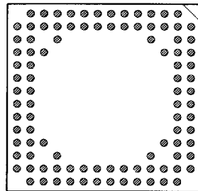
100 PINS PATTERN 1428
