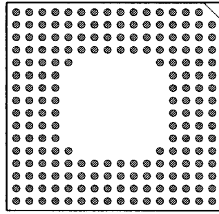
195 PINS PATTERN 1612
