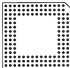
142 PINS PATTERN 1526
