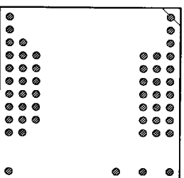
52 PINS PATTERN 1336
