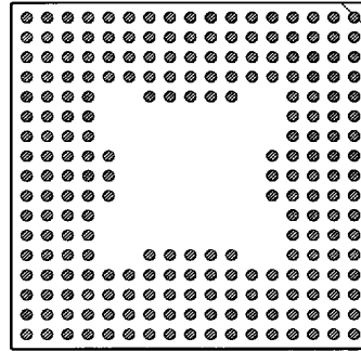
224 PINS PATTERN 1734
