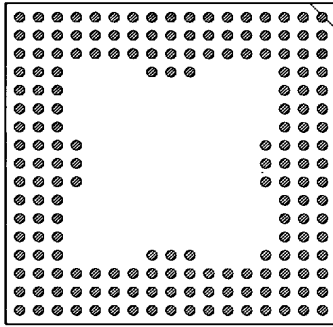
181 PINS PATTERN 1726
