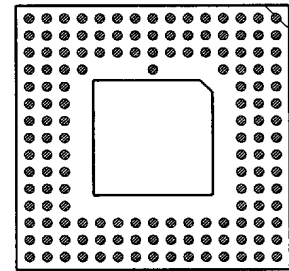
147 PINS PATTERN 1542
