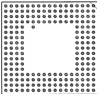
209 PINS PATTERN 1730
