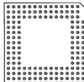
141 PINS PATTERN 1528
