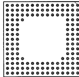
147 PINS PATTERN 1543
