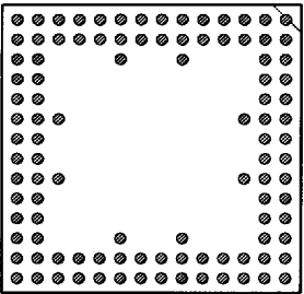
104 PINS PATTERN 1417
