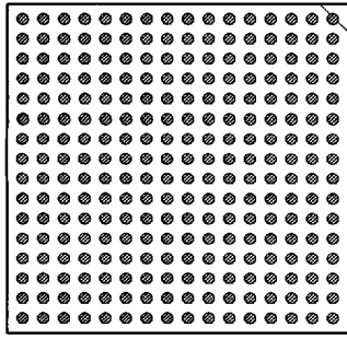
256 PINS PATTERN 1601
