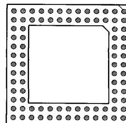
88 PINS PATTERN 1327
