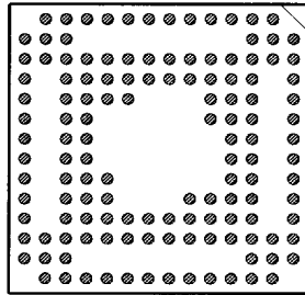
132 PINS PATTERN 1433
