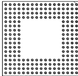
208 PINS PATTERN 1728
