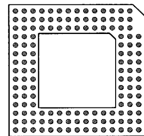
141 PINS PATTERN 1527
