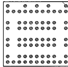
72 PINS PATTERN 1154
