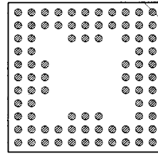
85 PINS PATTERN 1108
