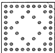
48 PINS PATTERN 0911
