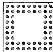
56 PINS PATTERN 0908
