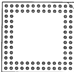
88 PINS PATTERN 1328
