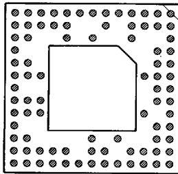
88 PINS PATTERN 1351
