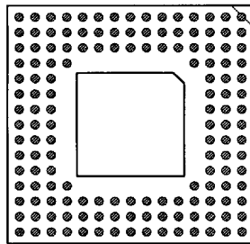
148 PINS PATTERN 1519
