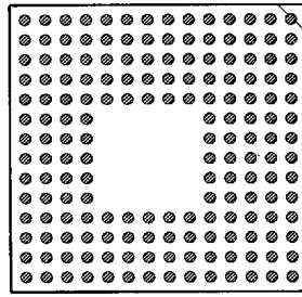
171 PINS PATTERN 1407
