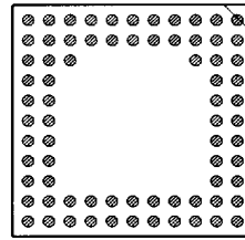
74 PINS PATTERN 1115
