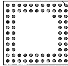
73 PINS PATTERN 1164
