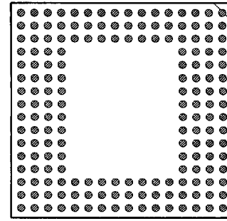
176 PINS PATTERN 1611
