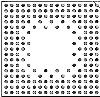
209 PINS PATTERN 1732
