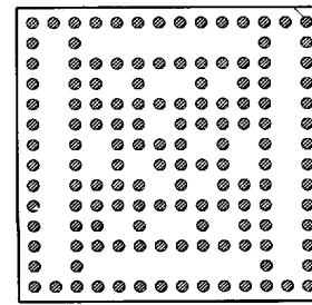
139 PINS PATTERN 1409
