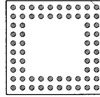
64 PINS PATTERN 1010
