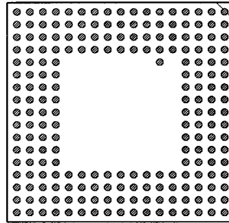
209 PINS PATTERN 1731
