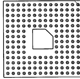
171 PINS PATTERN 1406
