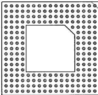
209 PINS PATTERN 1729
