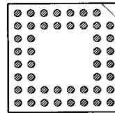
47 PINS PATTERN 0810
