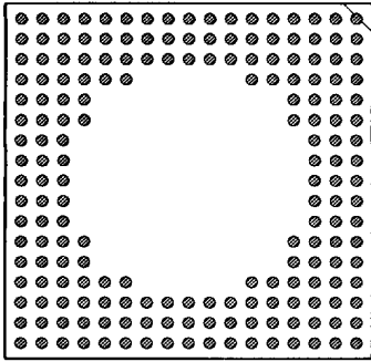
188 PINS PATTERN 1727
