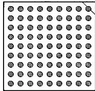
81 PINS PATTERN 0901
