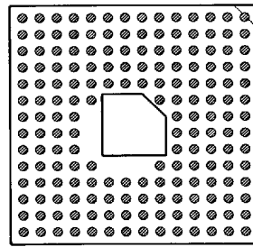
175 PINS PATTERN 1404
