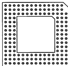
142 PINS PATTERN 1525
