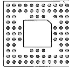
85 PINS PATTERN 1107
