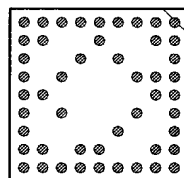
49 PINS PATTERN 0910
