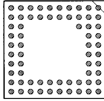
65 PINS PATTERN 1008
