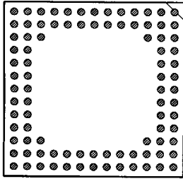
92 PINS PATTERN 1352
