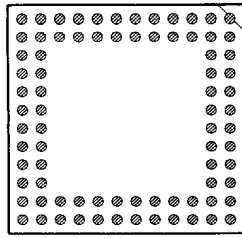
80 PINS PATTERN 1215
