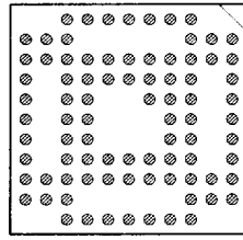
85 PINS PATTERN 1165
