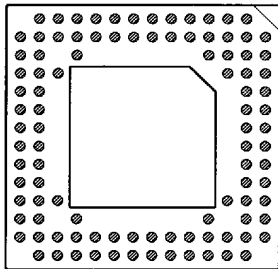
101 PINS PATTERN 1429
