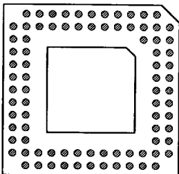
85 PINS PATTERN 1331
