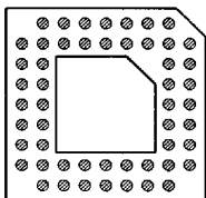
52 PINS PATTERN 0916
