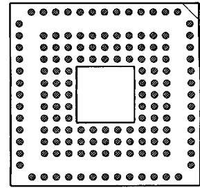
148 PINS PATTERN 1544
