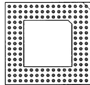
144 PINS PATTERN 1523
