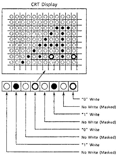
Figure 3. Corresponding bit-map
