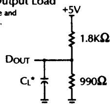
Figure 1. Output Load
