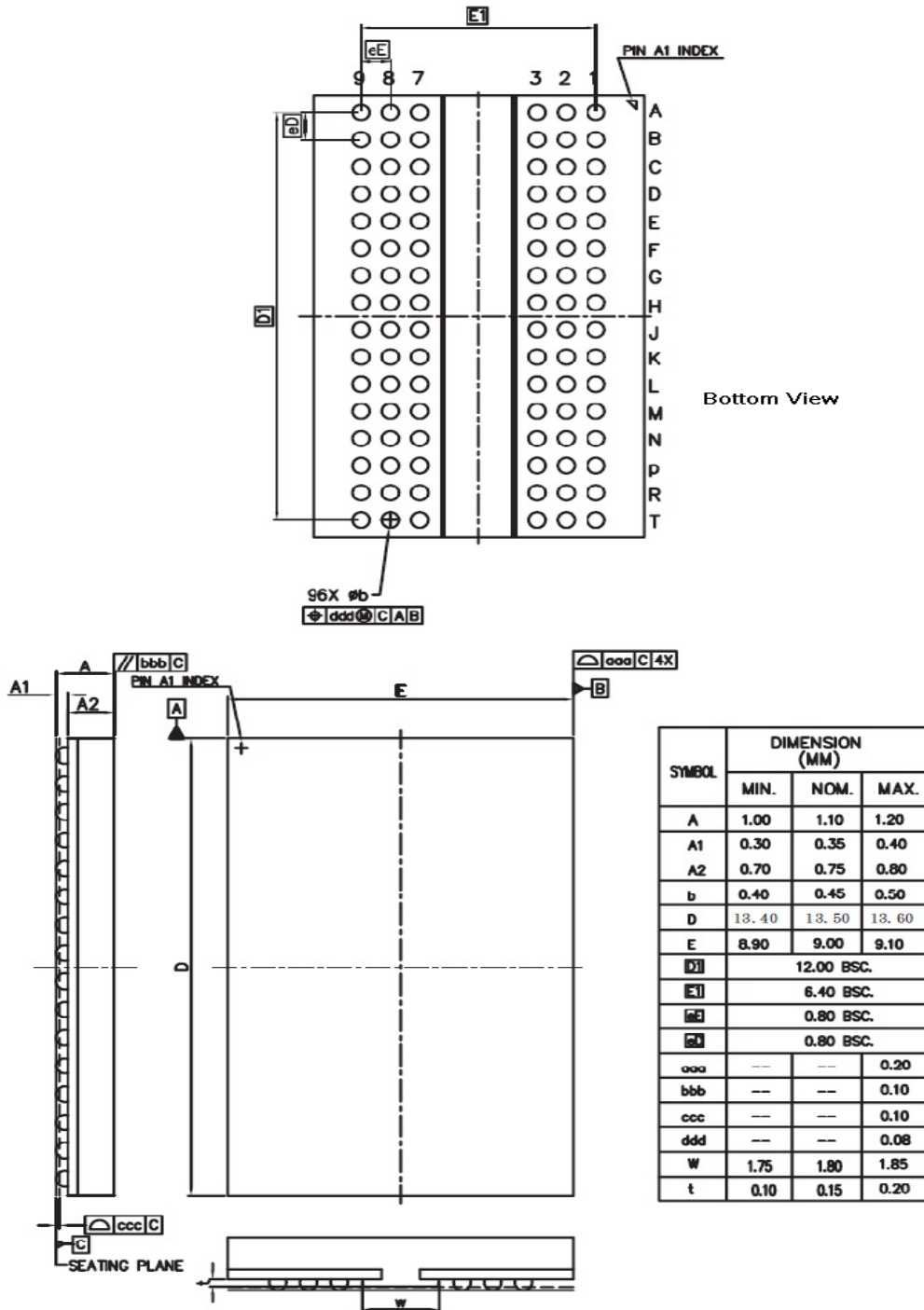
FIGURE 5 Package outline
