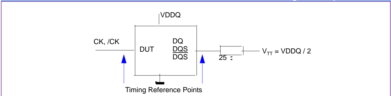
Reference Load for AC Timings and Output Slew Rates
