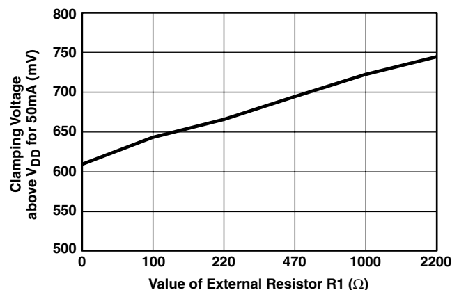
Figure 8. Clamping Voltage vs R1 @ V_{DD} = 3.3V
