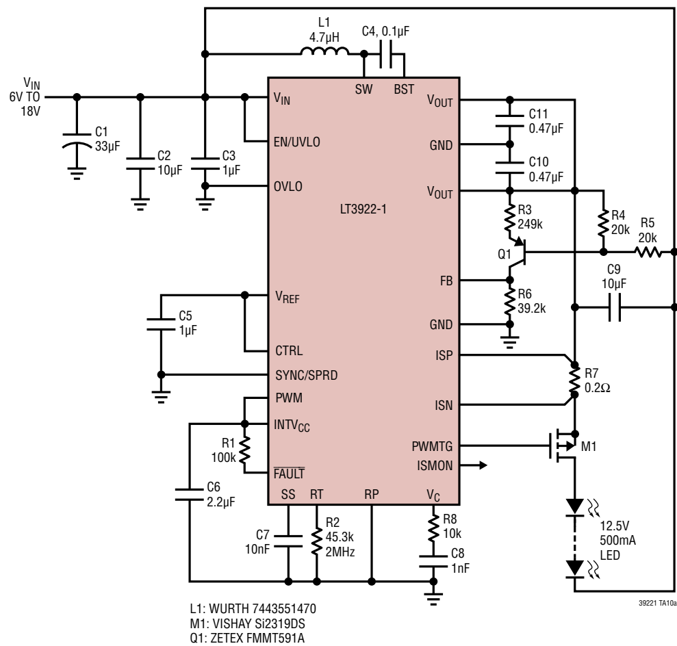
2MHz, 88% Efficient 6.25W (12.5V, 500mA) Buck-Boost Mode LED Driver
