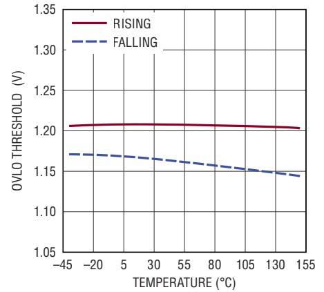
OVLO Threshold
