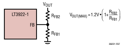
Figure 7. FB Resistor Configuration
