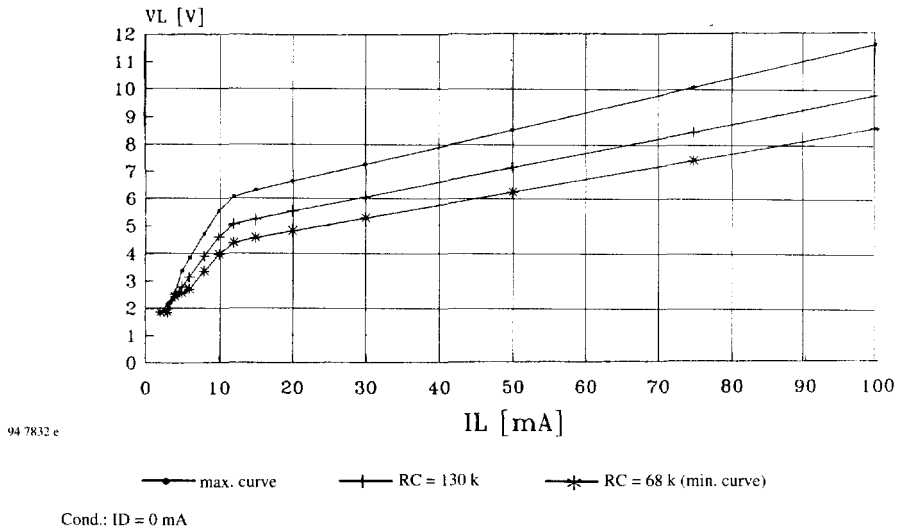
Figure 12. DC characteristics
