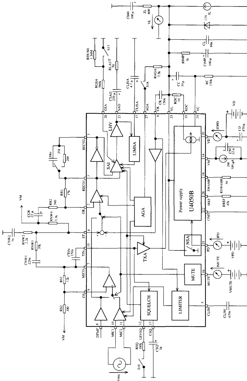
Figure 10. Test circuit for MUTE and PD test
