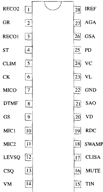
Figure 3. Pinning S028
