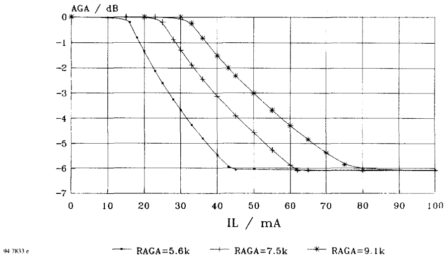
Figure 13. AGA characteristics
