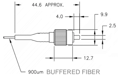
FC CONNECTOR FOR Ø 900µm BUFFERED FIBER
