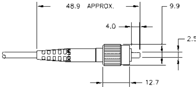
FC CONNECTOR FOR Ø 2.8mm CABLE
