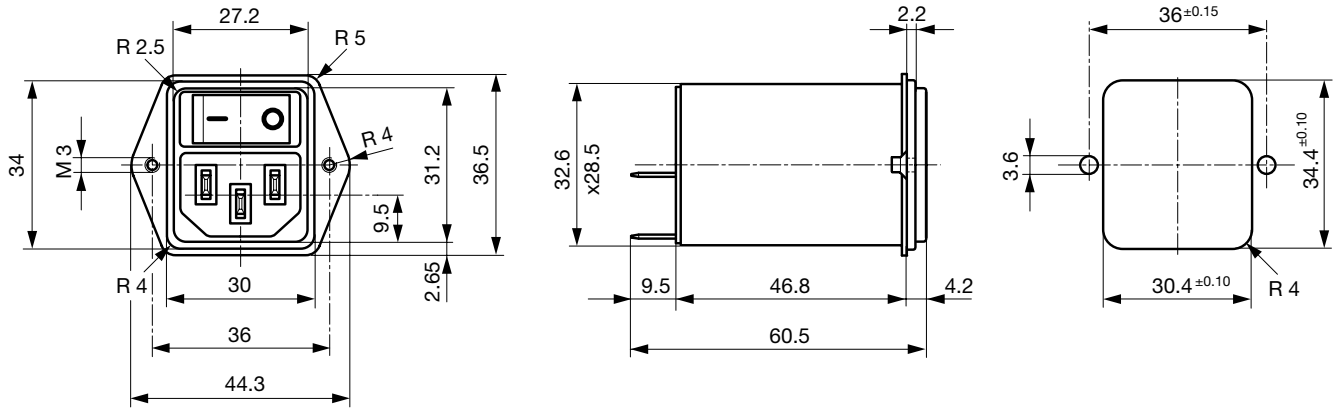
Screw-on mounting from front side (protection class II)
