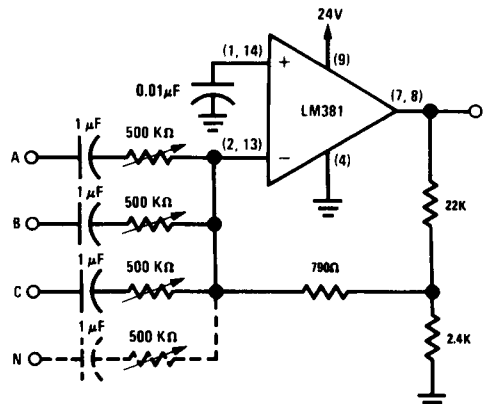
Audio Mixer
