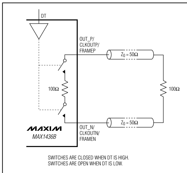
Figure 8. Double-Termination
