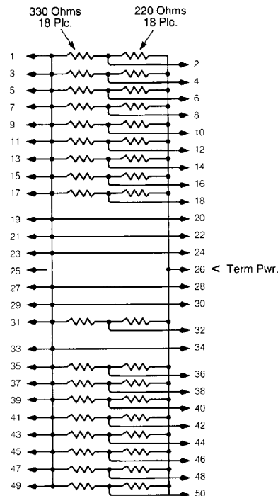
50-Position, Single-Ended Part No. 869647-1
